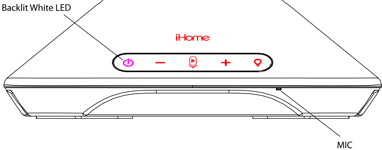
Milky Translucent Rubber Button Panel with Silk Screen Masked Graphics
