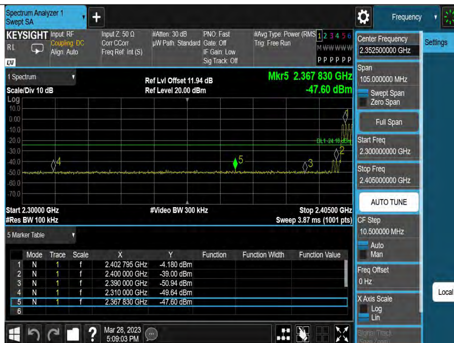
DH5-Ant1-Low-Hop_2402--4.18
