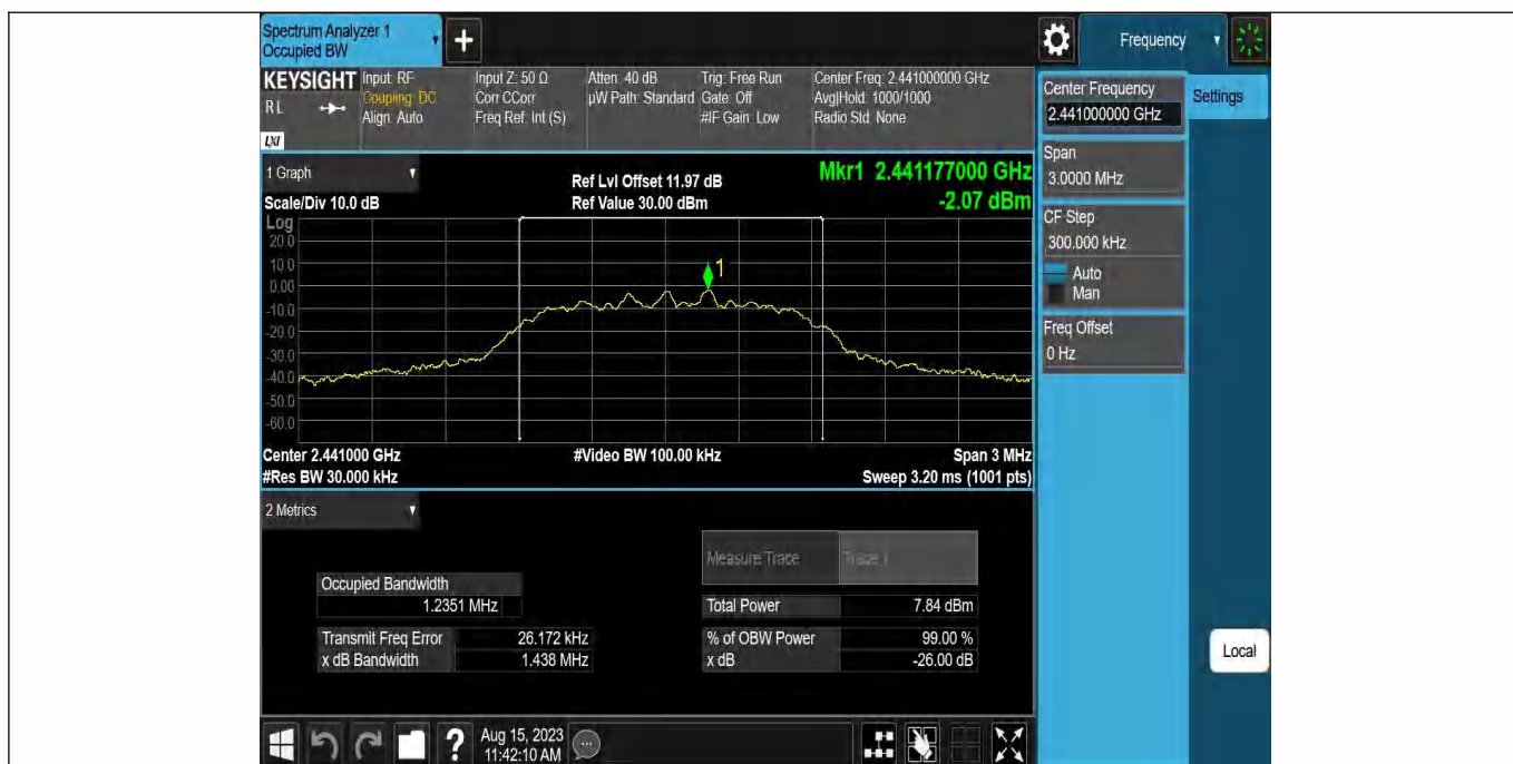
2DH5-Ant1-2441
