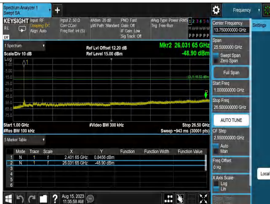
DH5-Ant1-2402-1000~26500
