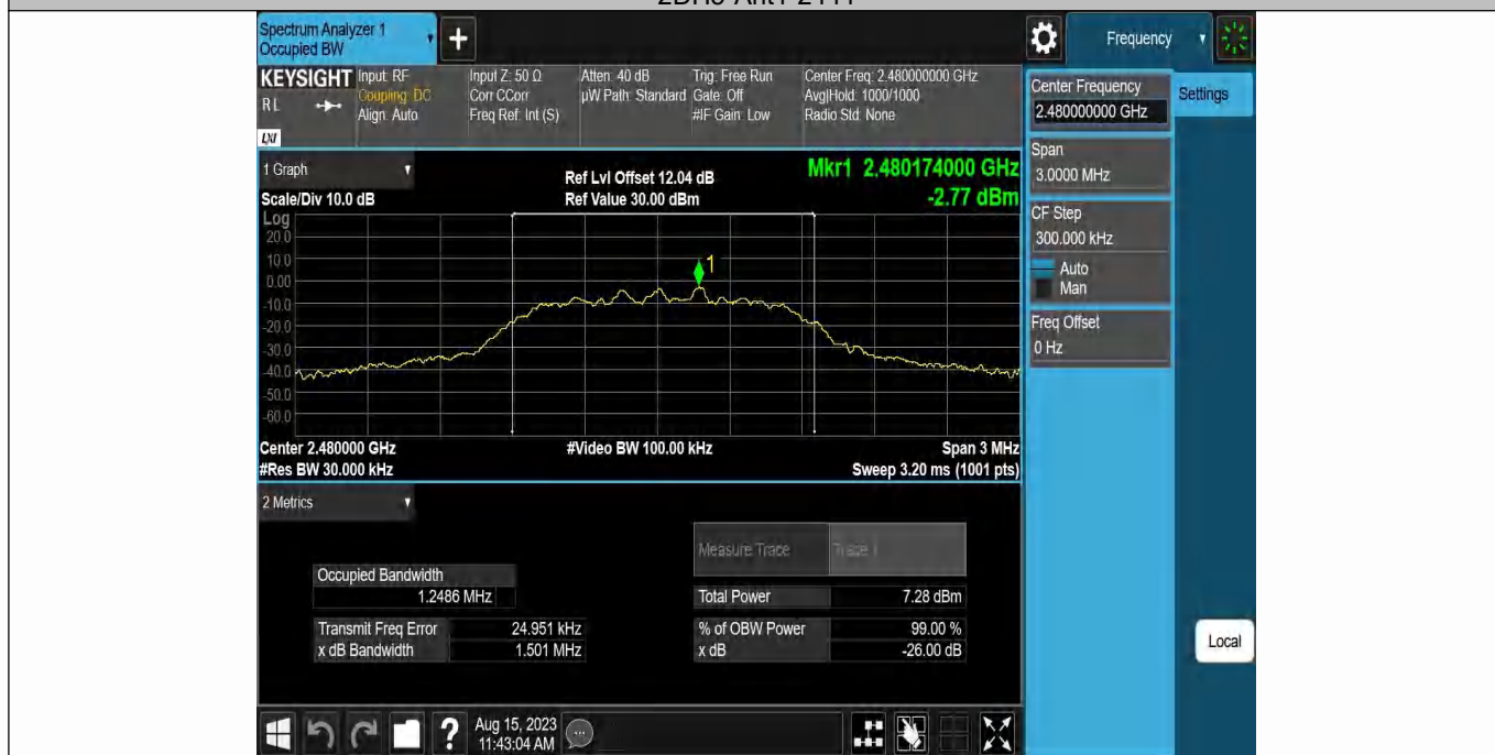
2DH5-Ant1-2480
