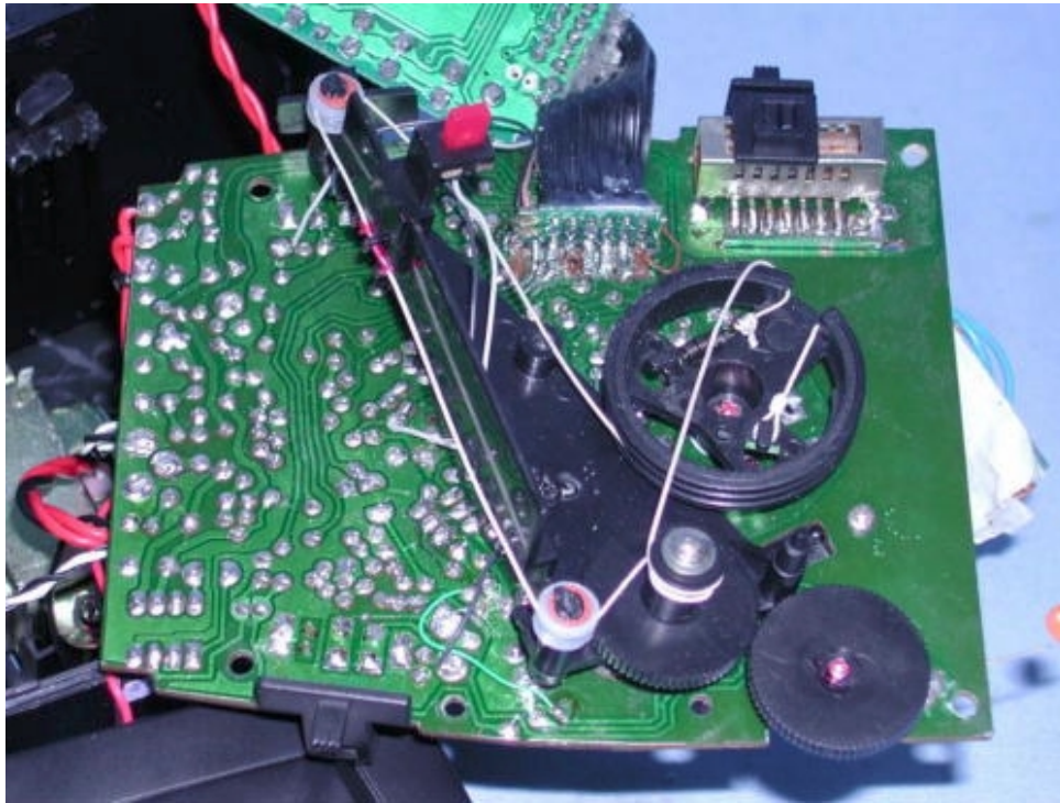
Main PCB solder side
