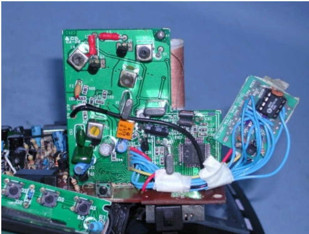
Other PCBs comp side
