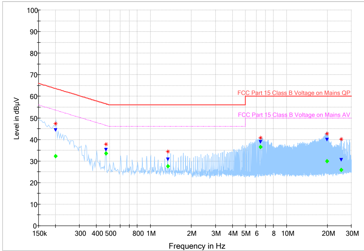
Figure 8.2-1: Conducted disturbance at mains port spectral plot (combination of neutral and line 1)
