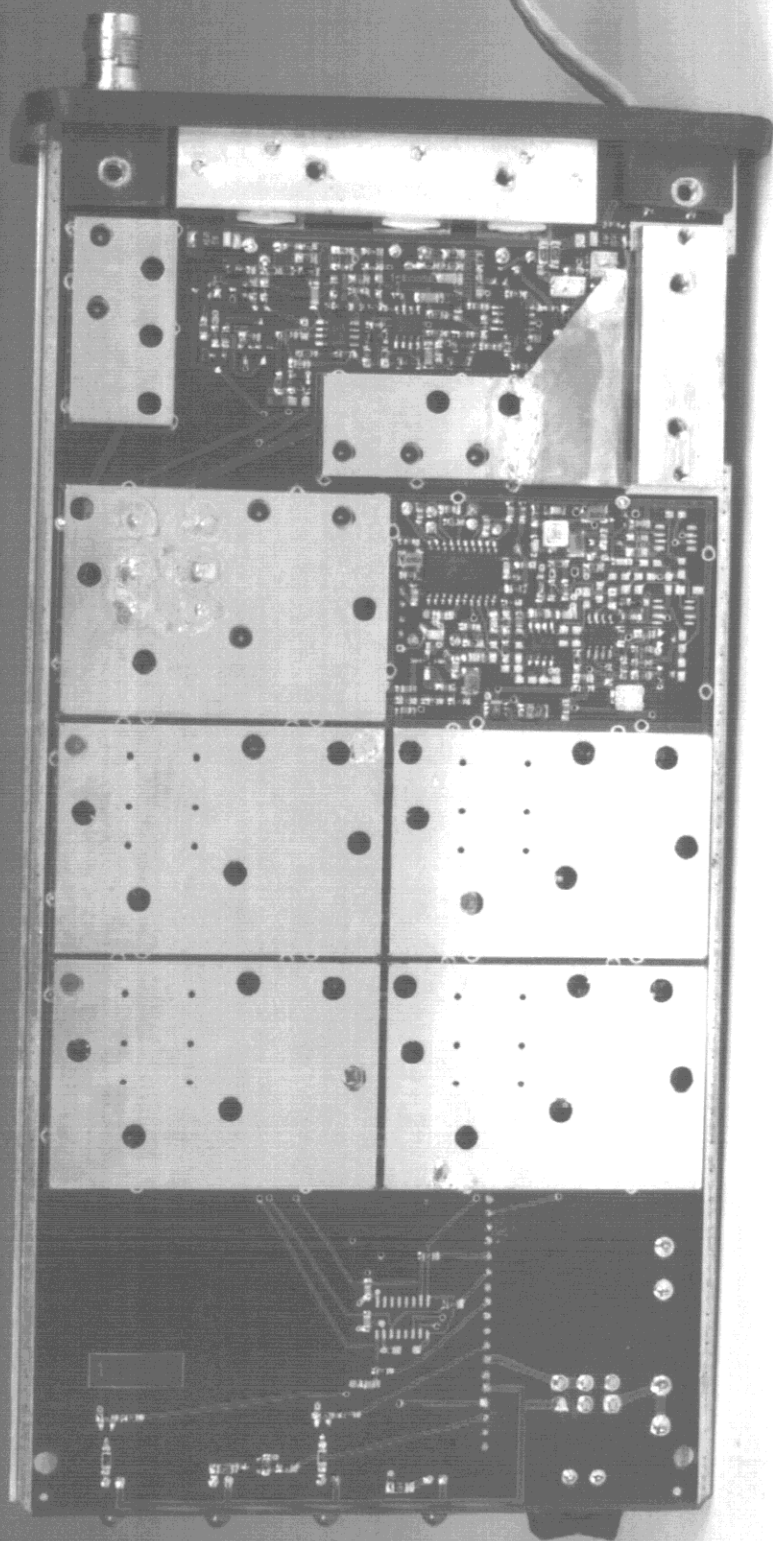
8R00570.1 ELECTRONIC SYSTEMS TECHNOLOGY ESTEEM 192M WIRELESS MODEM RF PCB BOTTOM WITH SHIELDS
