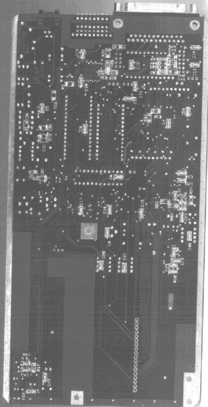
8R00570.1 ELECTRONIC SYSTEMS TECHNOLOGY ESTEEM 192M WIRELESS MODEM LOGIC PCB TRACE SIDE
