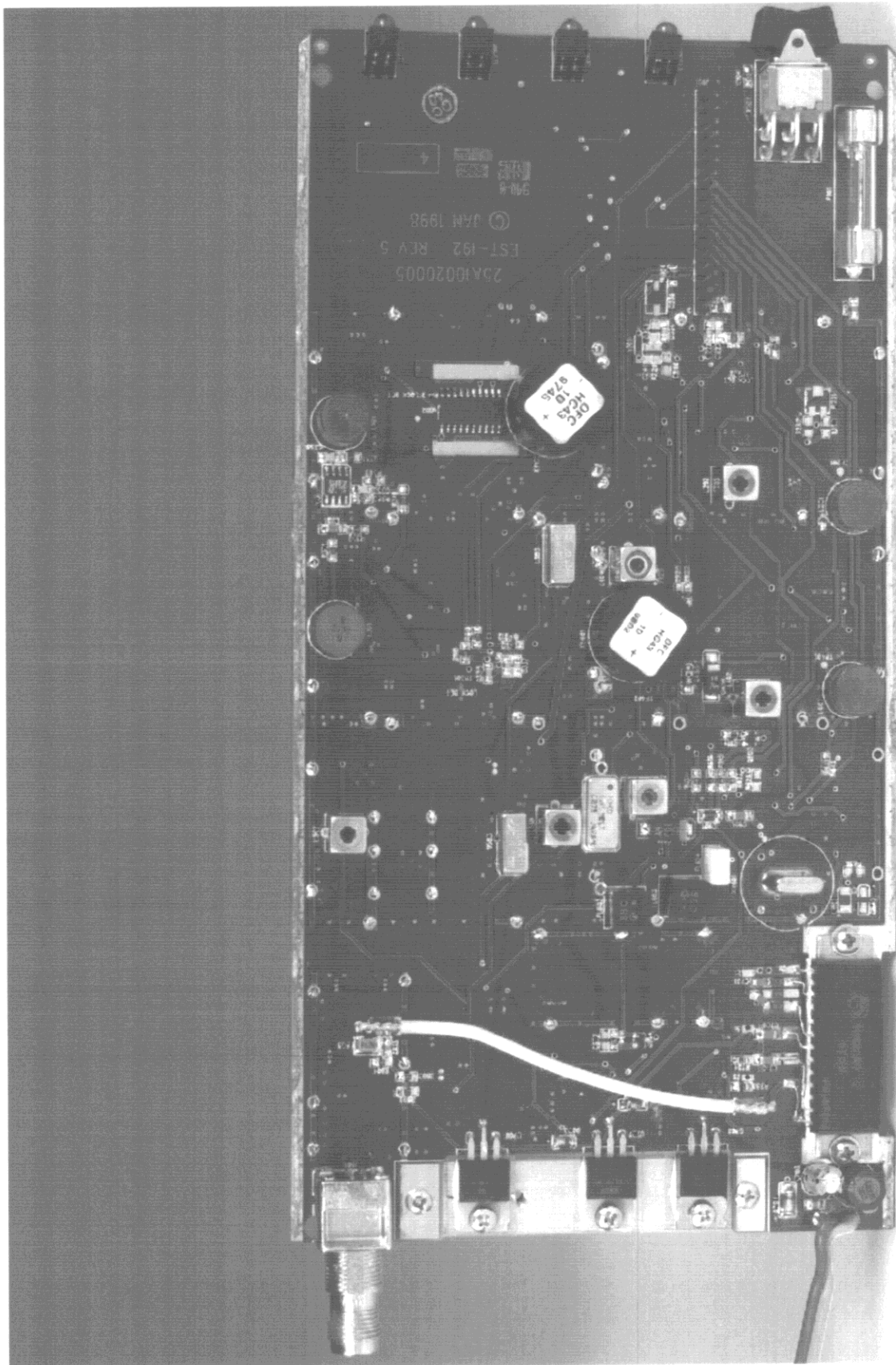
8R00570.1 ELECTRONIC SYSTEMS TECHNOLOGY ESTEEM 192M WIRELESS MODEM RF PCB TOP
