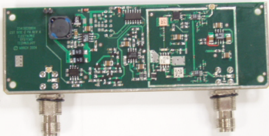
PA Board (Top)
