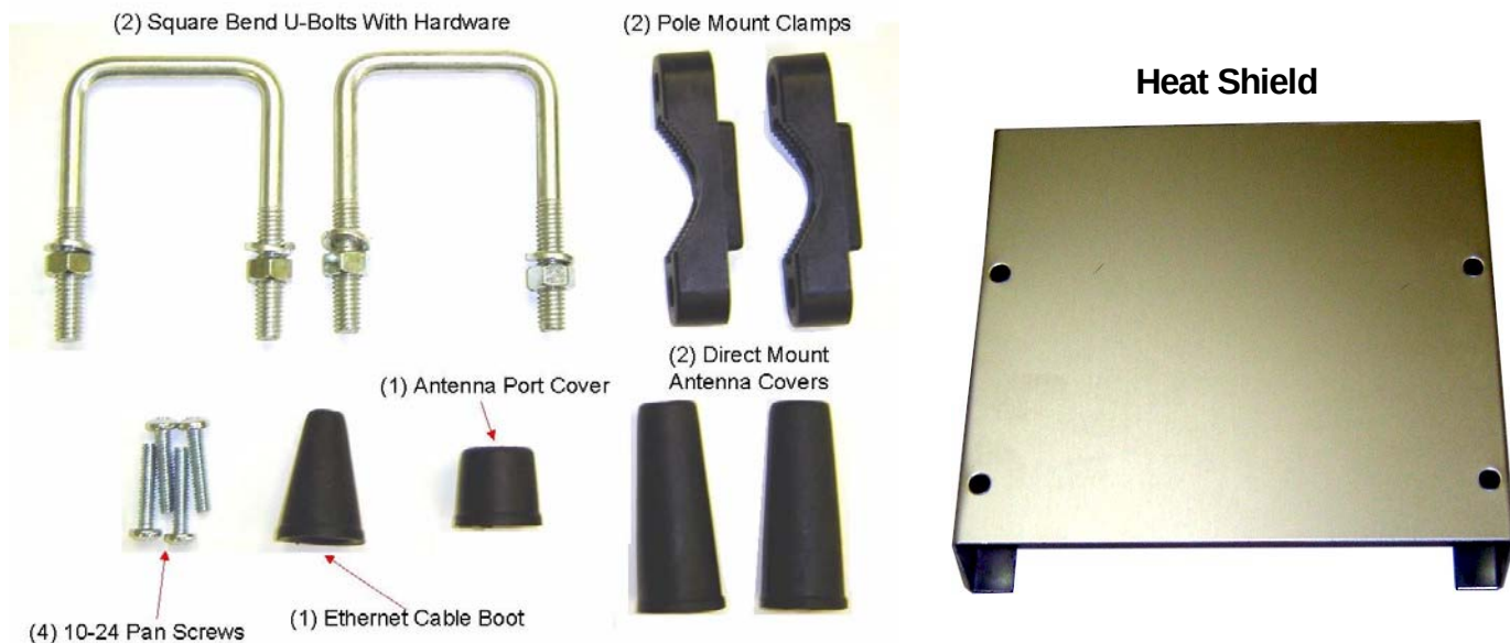
Figure 2: AA195PM Hardware Contents
