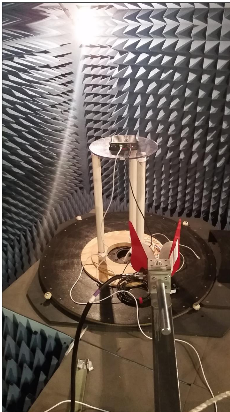
Photograph 5. Radiated Spurious Emissions, Test Setup, Above 1 GHz
