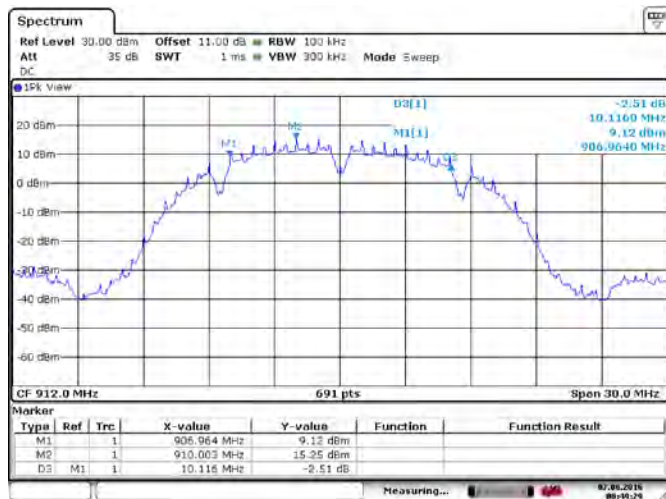
Figure 8.1-25: 6 dB bandwidth, 20MHz BW DSSS/BPSK 1 Mbps
