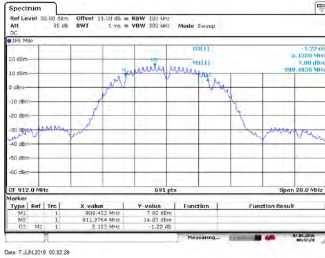
Figure 8.1-43: 6 dB bandwidth, 10MHz BW DSSS/BPSK 1 Mbps
