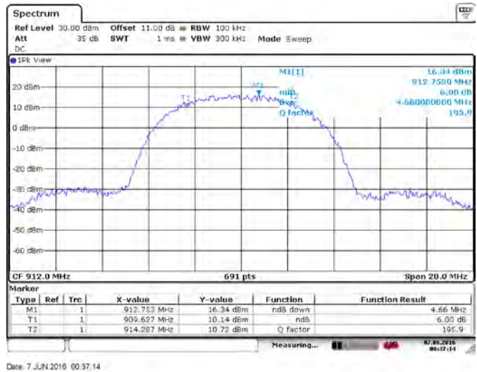
Figure 8.1-16: 6 dB bandwidth, 10MHz BW DSSS/CKK 11 Mbps
