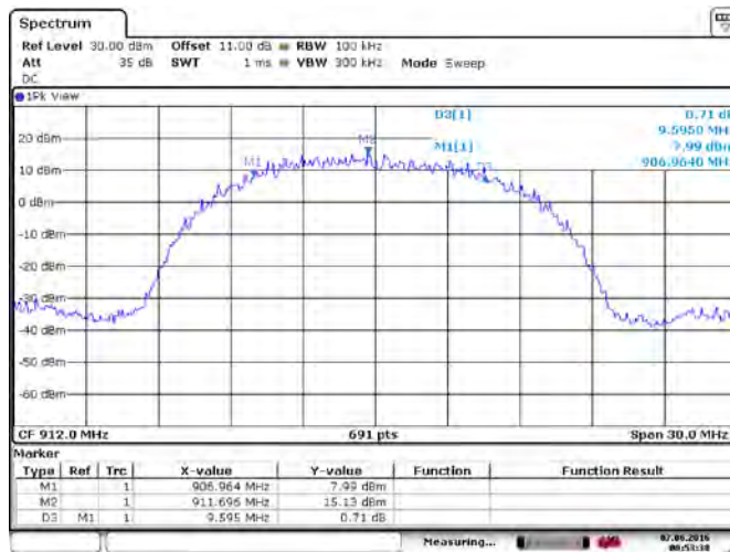
Figure 8.1-28: 6 dB bandwidth, 20MHz BW DSSS/CCK 11 Mbps
