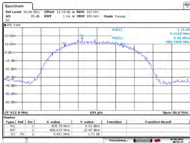
Figure 8.1-27: 6 dB bandwidth, 20MHz BW DSSS/CCK 5.5 Mbps
