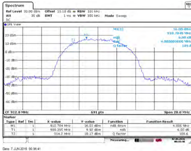
Figure 8.1-15: 6 dB bandwidth, 10MHz BW DSSS/CKK 5.5 Mbps
