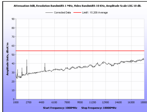
Plot 163. Radiated Spurious Emissions, Low Channel, 802.11b 10 MHz, Omni Antenna, 1 GHz – 18 GHz, Average
