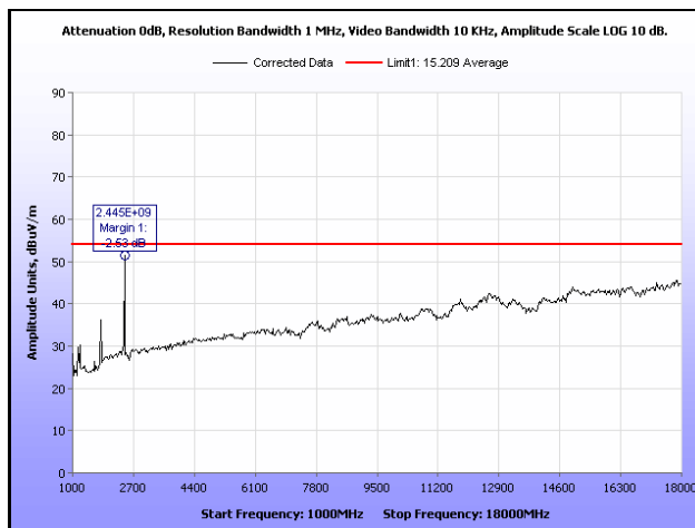
Plot 310. Radiated Spurious Emissions, Mid Channel, 802.11n 20 MHz, Parabolic Antenna, 1 GHz – 18 GHz, Average
