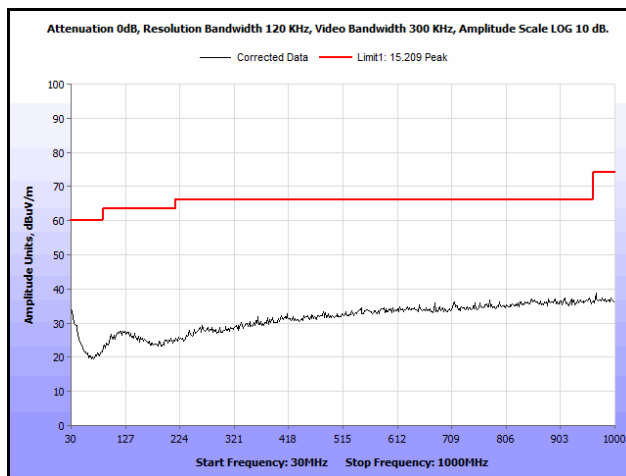
Plot 165. Radiated Spurious Emissions, Mid Channel, 802.11b 10 MHz, Omni Antenna, 30 MHz – 1 GHz
