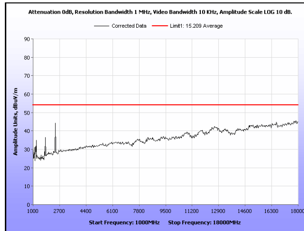
Plot 181. Radiated Spurious Emissions, Low Channel, 802.11n 10 MHz, Omni Antenna, 1 GHz – 18 GHz, Average
