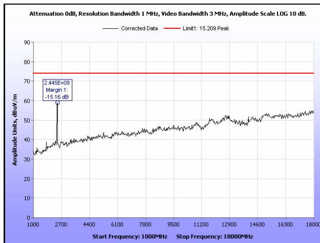
Plot 311. Radiated Spurious Emissions, Mid Channel, 802.11n 20 MHz, Parabolic Antenna, 1 GHz – 18 GHz, Peak
