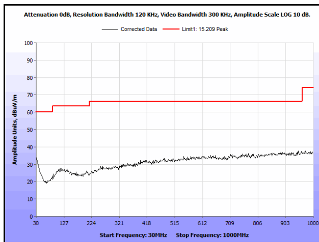
Plot 213. Radiated Spurious Emissions, High Channel, 802.11n 20 MHz, Omni Antenna, 30 MHz – 1 GHz
