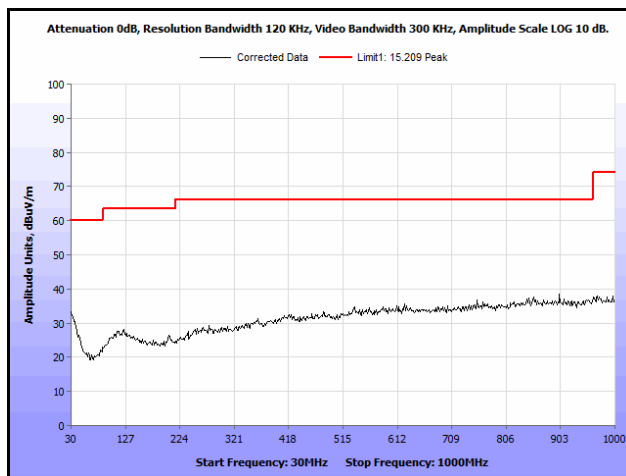
Plot 192. Radiated Spurious Emissions, Mid Channel, 802.11b 20 MHz, Omni Antenna, 30 MHz – 1 GHz
