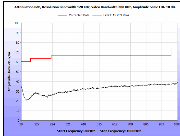
Plot 363. Radiated Spurious Emissions, Mid Channel, 802.11b 10 MHz, Yagi Antenna, 30 MHz – 1 GHz
