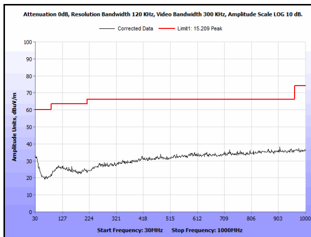
Plot 339. Radiated Spurious Emissions, High Channel, 802.11b 5 MHz, Yagi Antenna, 30 MHz – 1 GHz
