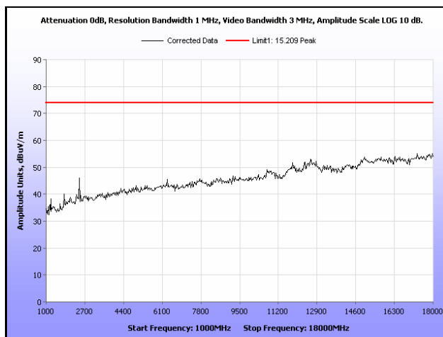
Plot 188. Radiated Spurious Emissions, High Channel, 802.11n 10 MHz, Omni Antenna, 1 GHz – 18 GHz, Peak
