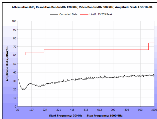
Plot 282. Radiated Spurious Emissions, Mid Channel, 802.11n 10 MHz, Parabolic Antenna, 30 MHz – 1 GHz
