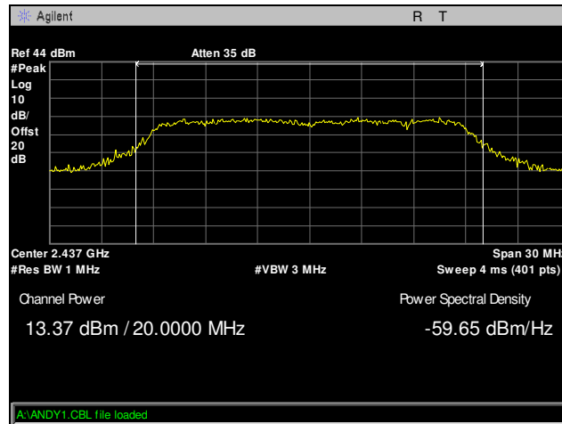
Plot 94. Peak Power Output, Mid Channel, 802.11n 20 MHz, Parabolic Antenna
