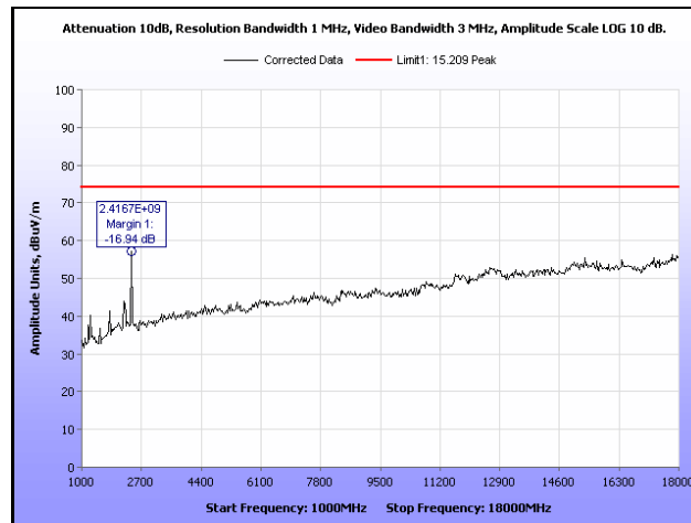
Plot 380. Radiated Spurious Emissions, Low Channel, 802.11n 10 MHz, Yagi Antenna, 1 GHz – 18 GHz, Peak
