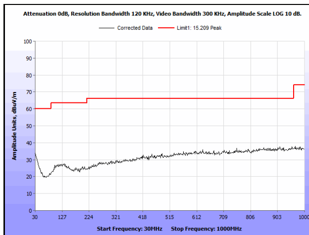
Plot 144. Radiated Spurious Emissions, Low Channel, 802.11g 5 MHz, Omni Antenna, 30 MHz – 1 GHz
