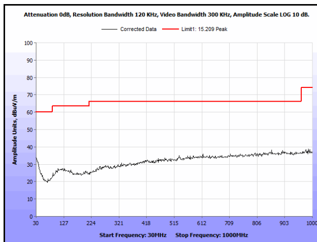
Plot 309. Radiated Spurious Emissions, Mid Channel, 802.11n 20 MHz, Parabolic Antenna, 30 MHz – 1 GHz
