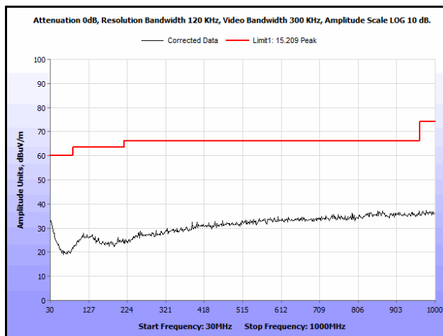
Plot 318. Radiated Spurious Emissions, Mid Channel, 802.11g 40 MHz, Parabolic Antenna, 30 MHz – 1 GHz
