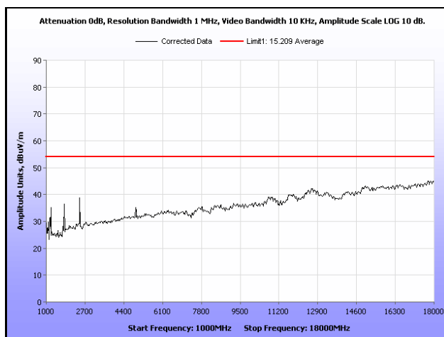
Plot 187. Radiated Spurious Emissions, High Channel, 802.11n 10 MHz, Omni Antenna, 1 GHz – 18 GHz, Average
