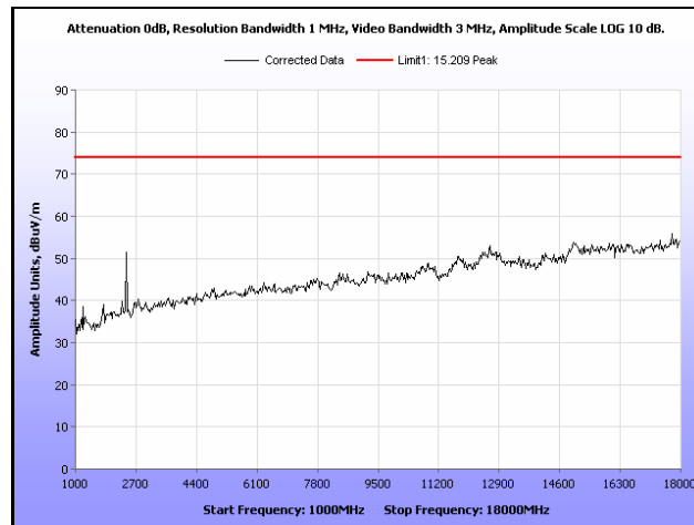
Plot 182. Radiated Spurious Emissions, Low Channel, 802.11n 10 MHz, Omni Antenna, 1 GHz – 18 GHz, Peak
