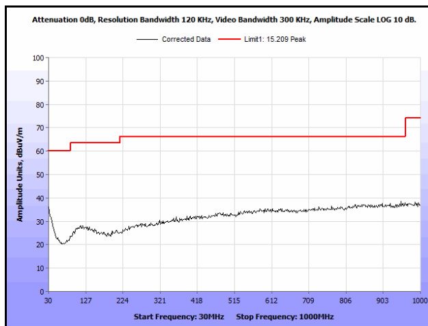
Plot 168. Radiated Spurious Emissions, High Channel, 802.11b 10 MHz, Omni Antenna, 30 MHz – 1 GHz
