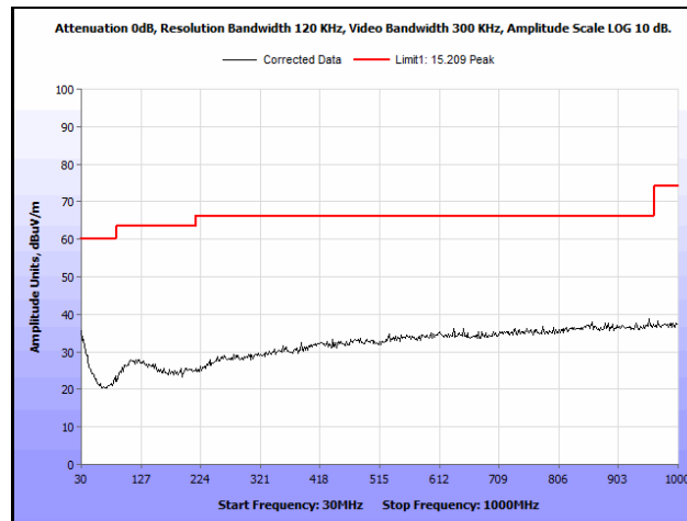
Plot 351. Radiated Spurious Emissions, Low Channel, 802.11n 5 MHz, Yagi Antenna, 30 MHz – 1 GHz
