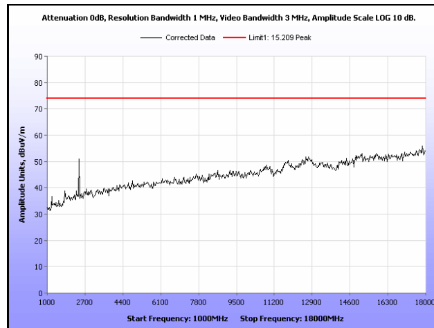
Plot 164. Radiated Spurious Emissions, Low Channel, 802.11b 10 MHz, Omni Antenna, 1 GHz – 18 GHz, Peak
