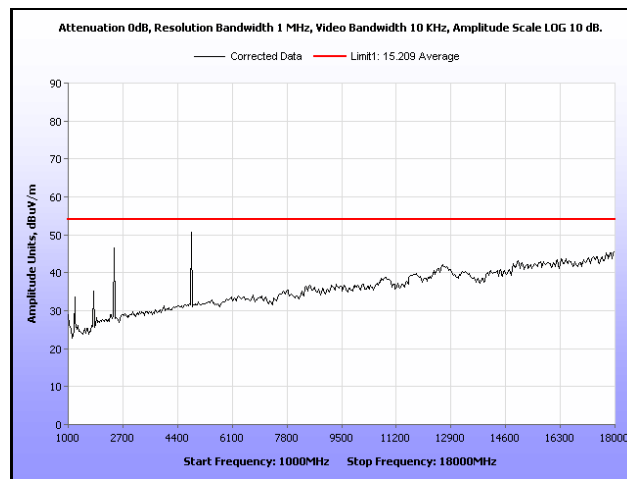
Plot 190. Radiated Spurious Emissions, Low Channel, 802.11b 20 MHz, Omni Antenna, 1 GHz – 18 GHz, Average
