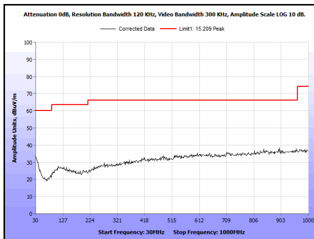
Plot 159. Radiated Spurious Emissions, High Channel, 802.11n 5 MHz, Omni Antenna, 30 MHz – 1 GHz
