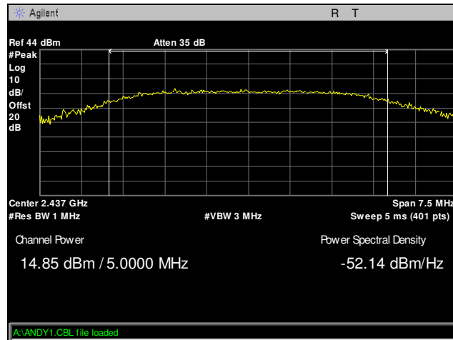
Plot 73. Peak Power Output, Mid Channel, 802.11g 5 MHz, Parabolic Antenna
