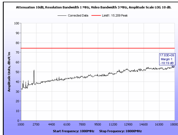
Plot 425. Radiated Spurious Emissions, Low Channel, 802.11n 40 MHz, Yagi Antenna, 1 GHz – 18 GHz, Peak
