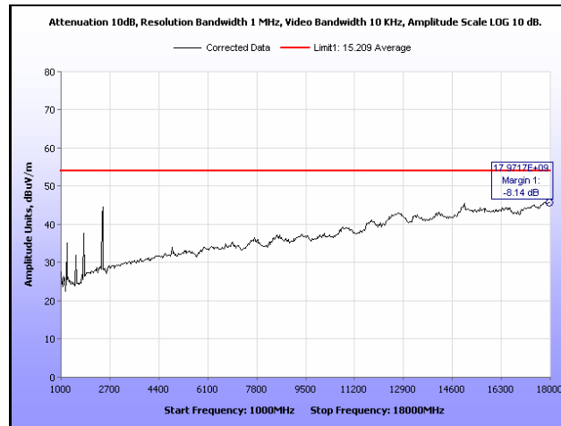
Plot 424. Radiated Spurious Emissions, Low Channel, 802.11n 40 MHz, Yagi Antenna, 1 GHz – 18 GHz, Average
