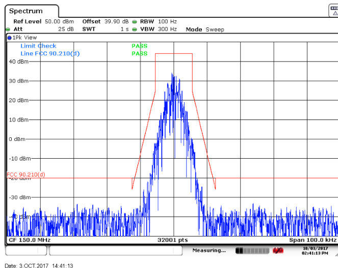
Emissions Mask ch150 MHz 12.5KHz dev 2000
