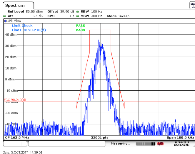
Emissions Mask ch162 MHz 12.5KHz dev 2000
