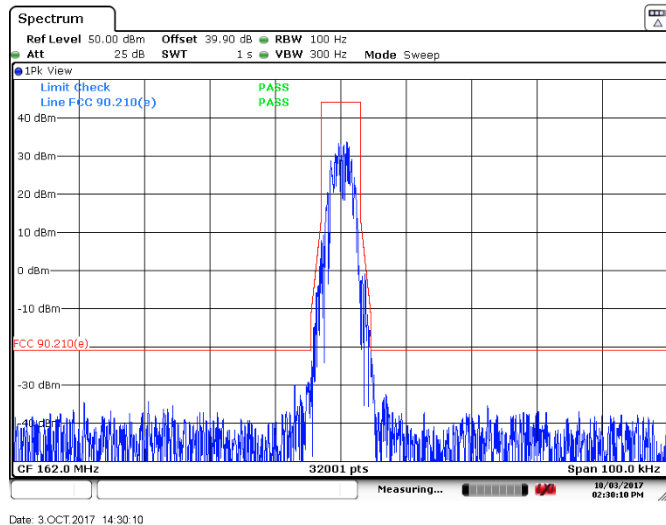
Emissions Mask ch162 MHz 6.25KHz dev 1500
