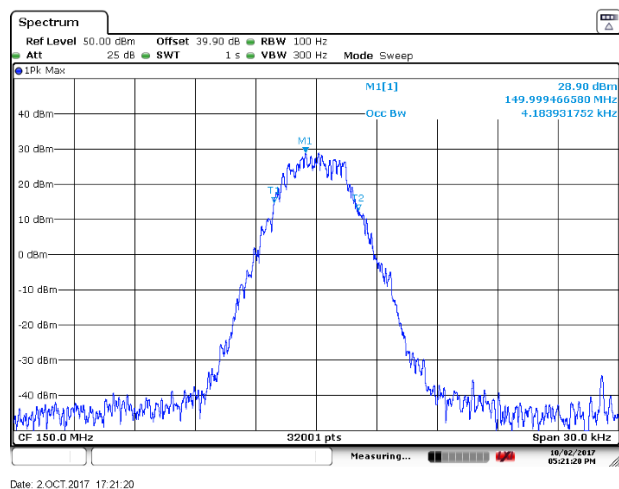
Input Signal (provided by 195M Transceiver)
