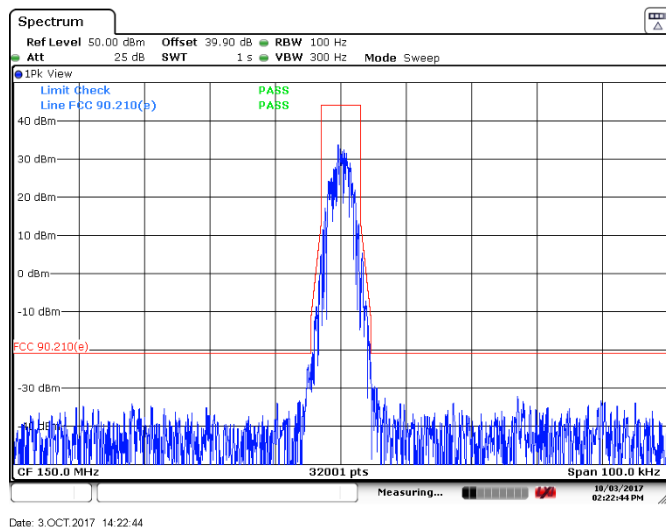
Emissions Mask ch150 MHz 6.2KHz dev 1500
