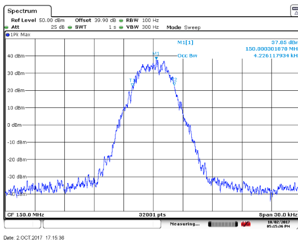
Output Signal (Amplifier Output)
