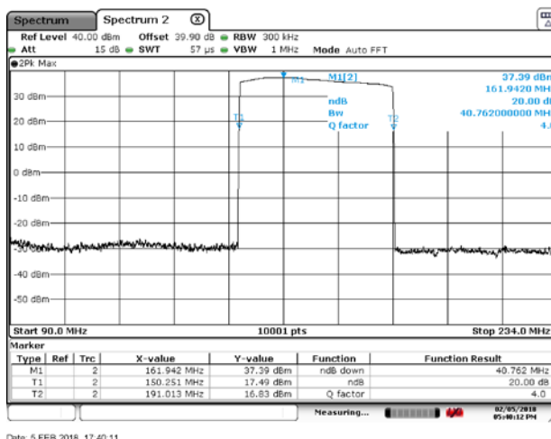
Amplifier Output
