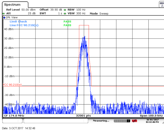
Emissions Mask ch174 MHz 6.25KHz dev 1500
