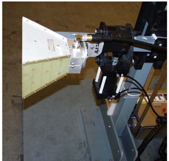
Photo 14 Alignment of the Center of Antenna with the Platform Edge
