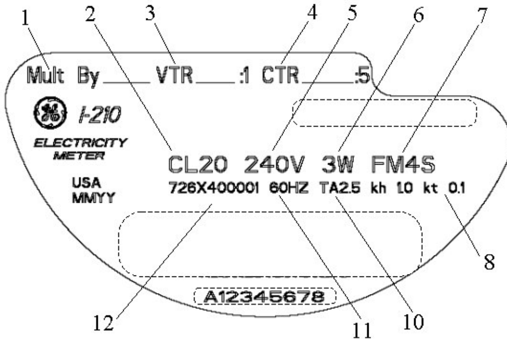
Figure 2-3: Nameplate
