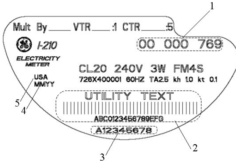
Figure 2-2. Nameplate Information
