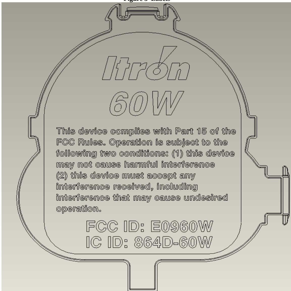
Figure 4 Stamped Endcap
