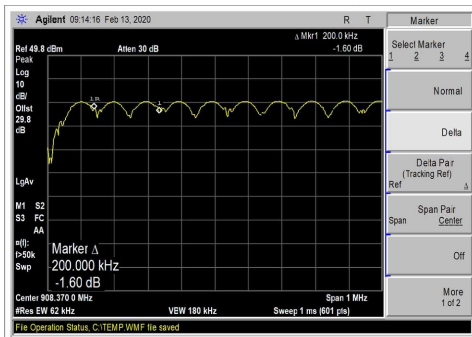
Carrier Separation
