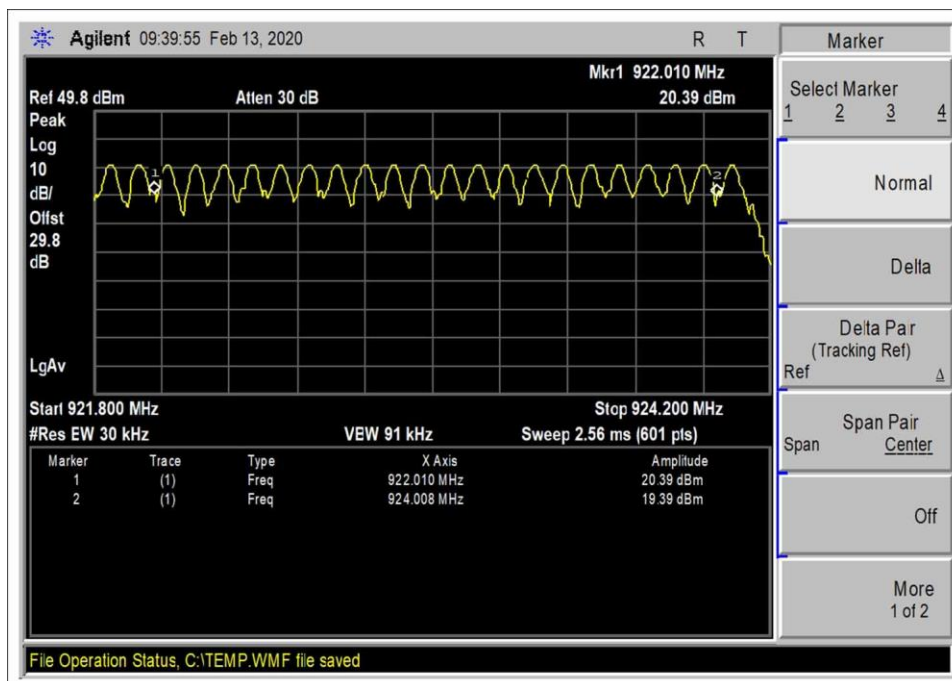
922-924MHz - 11 Channel
