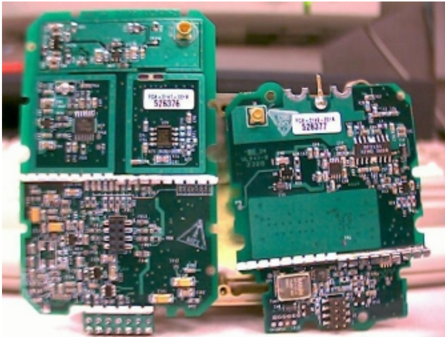
RX board picture rear out of module
