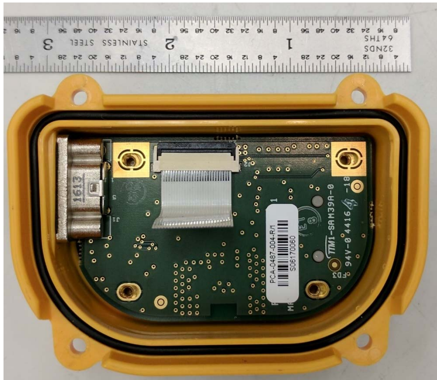
Communications Control Board - PCA-0487-00x
