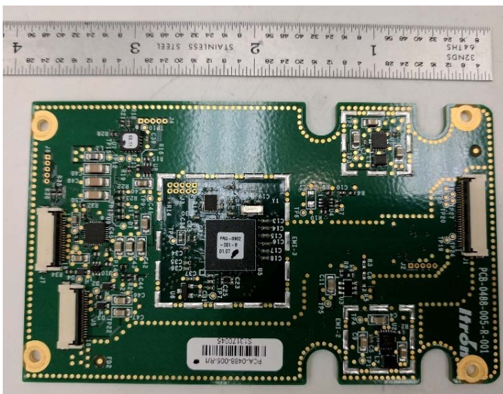
Host/Battery/USB Board - PCA-0488-00x
