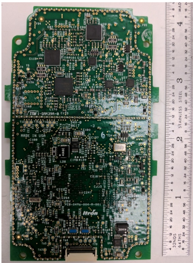
Single Board Super Raptor Radio Board - PCA-0496-00x
