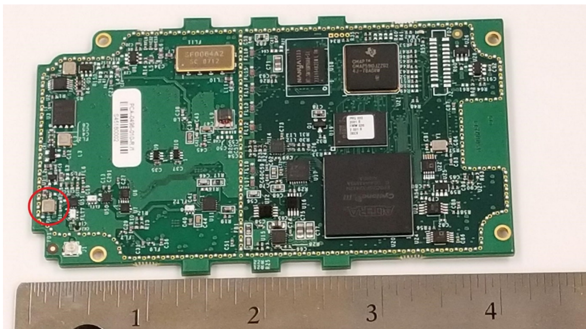
Filter FL1 (circled) not used on IMRB-EXT radio
