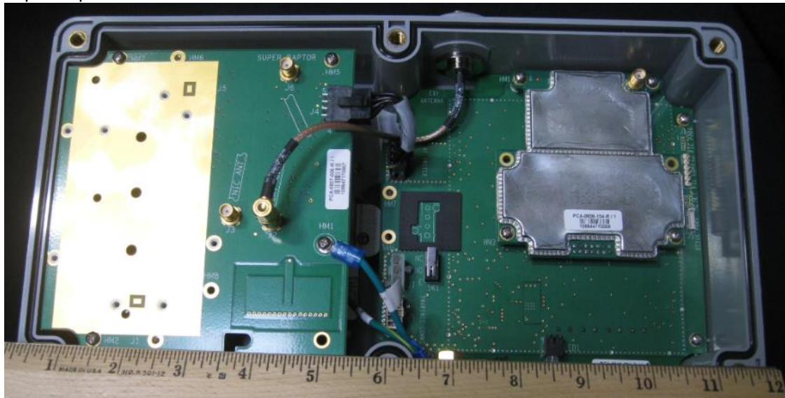
Super Raptor Radio Board
