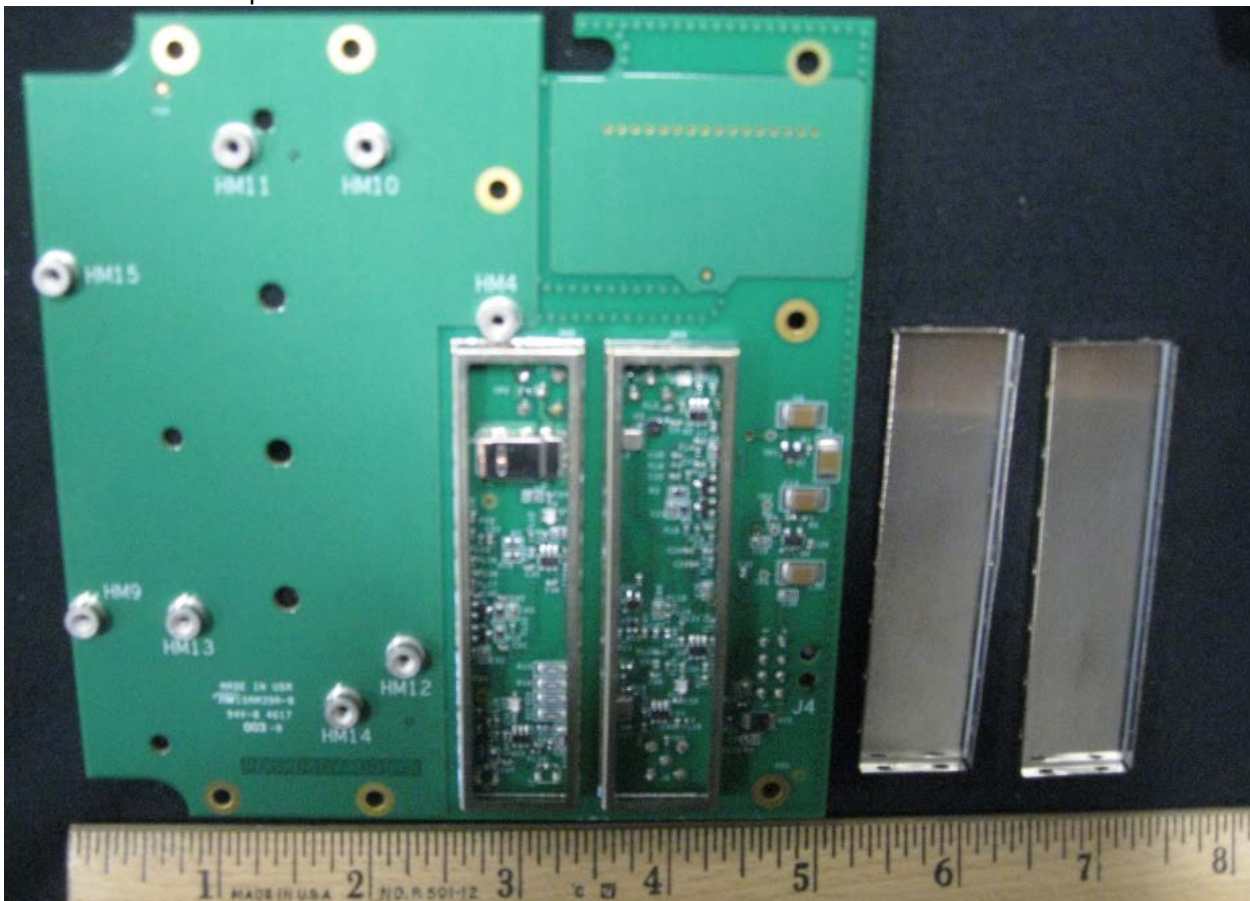
RF Switch Board - Bottom View
