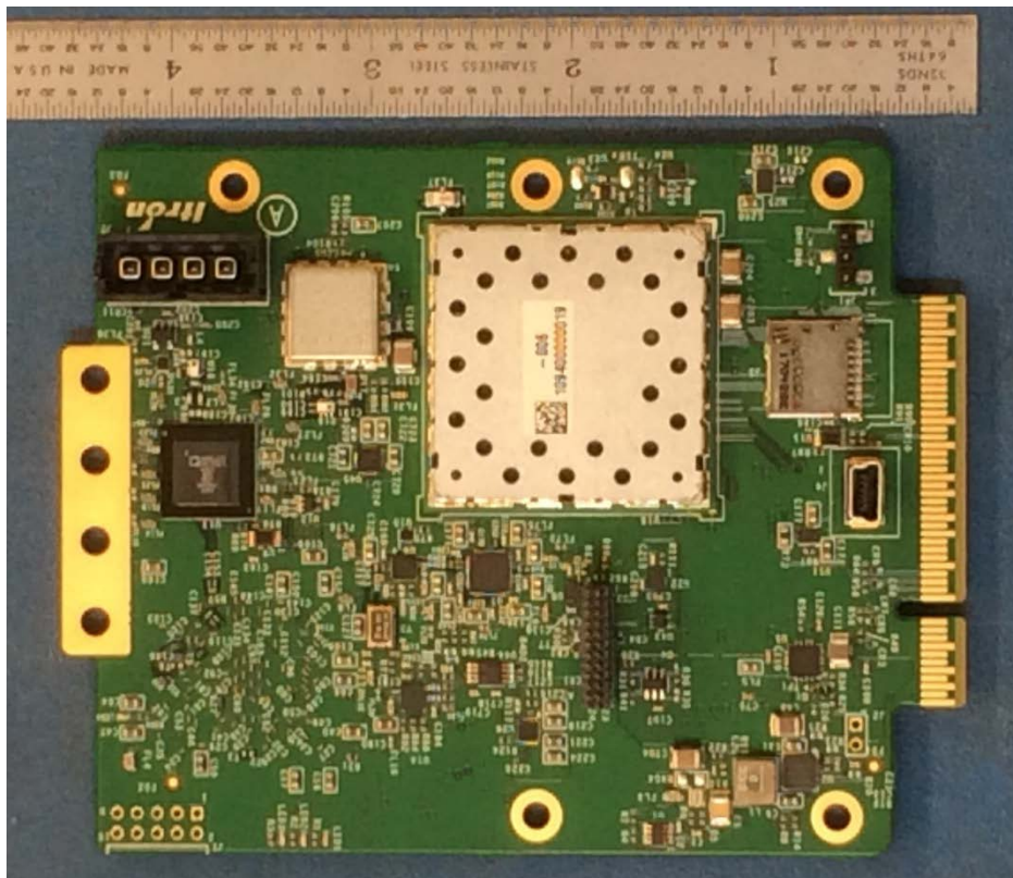
main board top with shield
