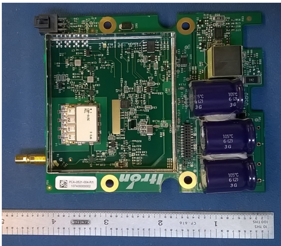
RF board top
