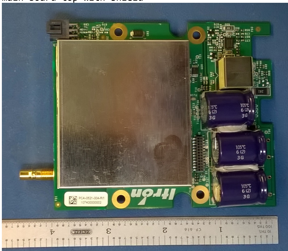
RF board top with shield
