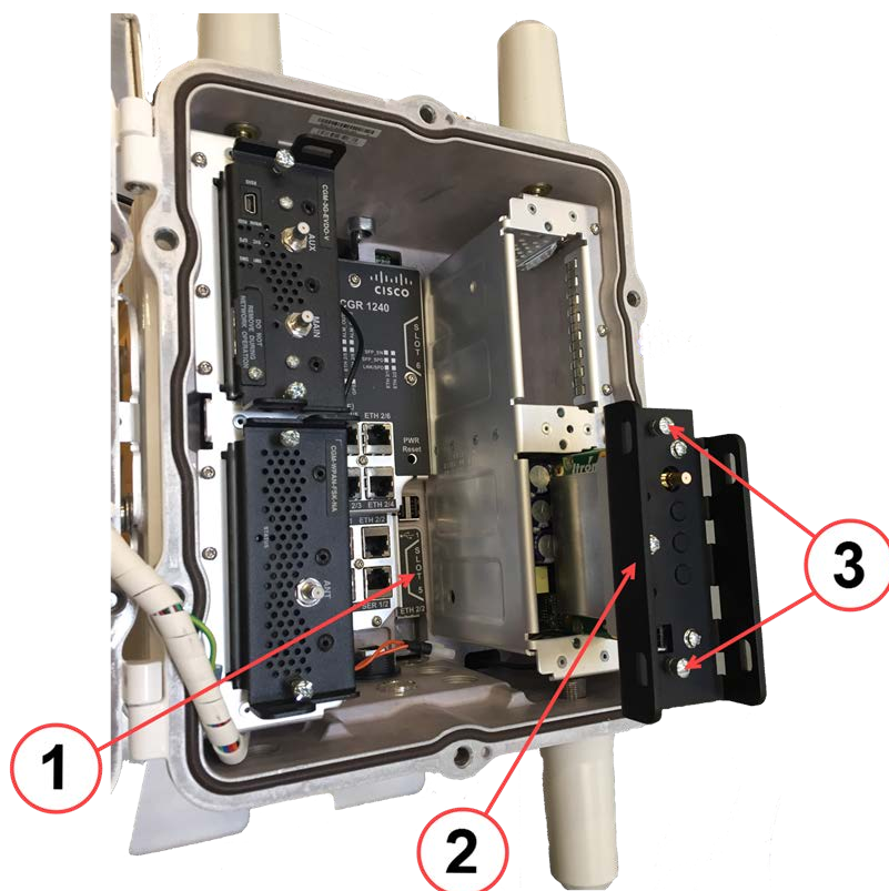
Figure 17 CGR's Slot 5 and CAM3M's Retaining Screws Location
