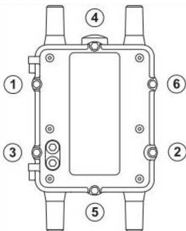
Figure 73 Six Captive Bolt Sequence to Loosen the CGR's Door
