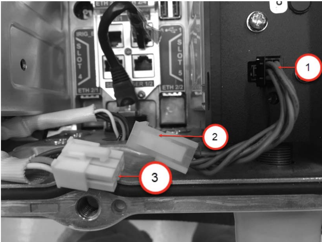
Figure 85 Using the Bulkhead Connector Assembly Extension Cable
