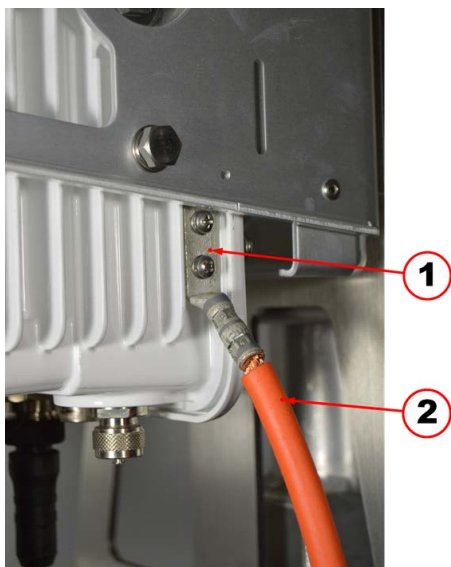
Figure 14 6AWG Ground Cable and Ground Lug Location
