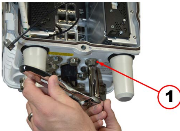
Figure 50 Hex Bolt Plug Location for PLC Signal Cable
