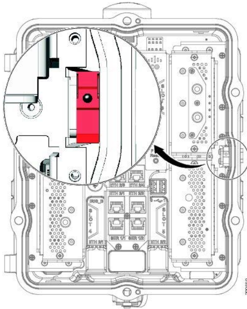
Figure 41 CGR's Door Sensor Location
