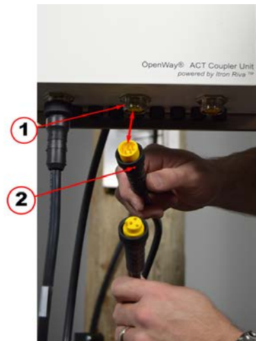
Figure 68 Power Output Connection Location
