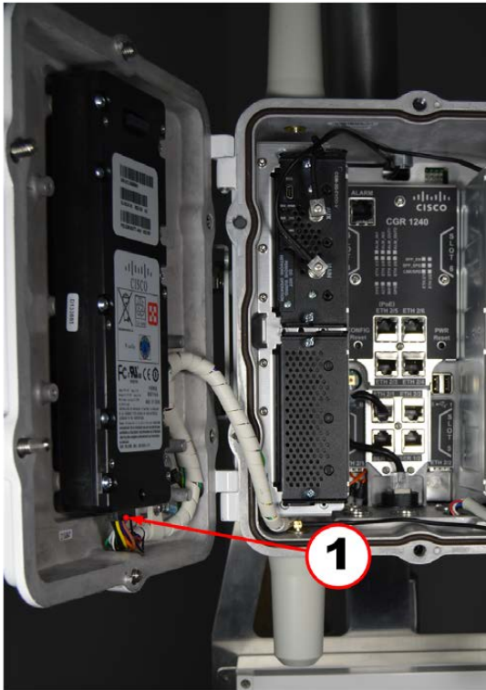
Figure 42 Battery Backup Unit (BBU) Harness Cable Connection Location
