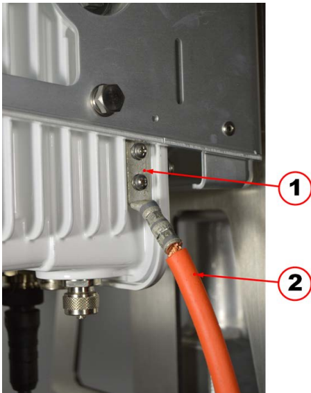
Figure 58 6AWG Ground Cable and Ground Lug Location
