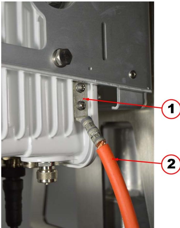
Figure 72 Ground Cable and Lug Screws Location
