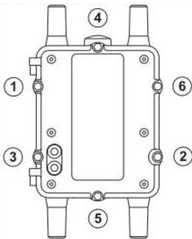
Figure 40 Six Captive Sequence to Loosen the CGR's Door
