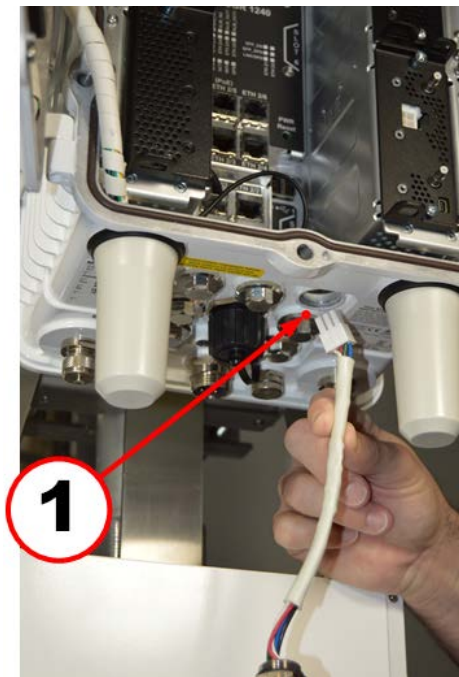
Figure 51 PLC Signal Cable Insertion Location
