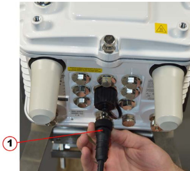
Figure 44 AC Power Cable Connection Location
