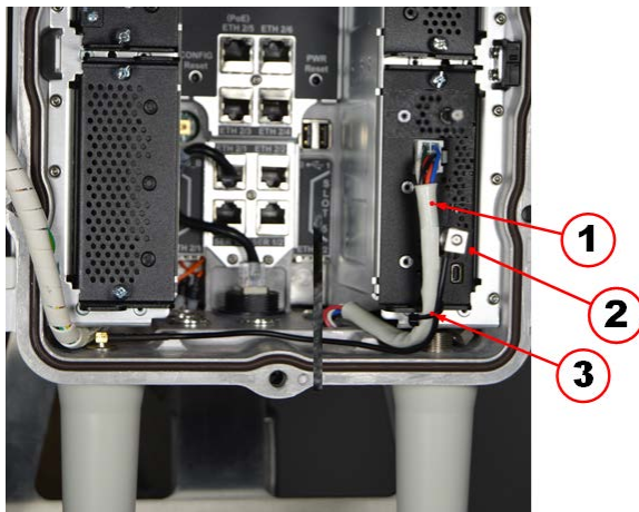
Figure 55 Signal Cable, RF Antenna Cable and Plastic Cable Tie Location
