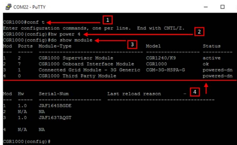
Figure 81 PuTTY Screen - Power Down CAM
