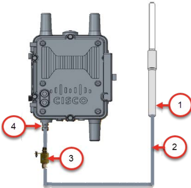
Figure 25 Remote Antenna, Lighting Arrestor Connections without a RF Filter
