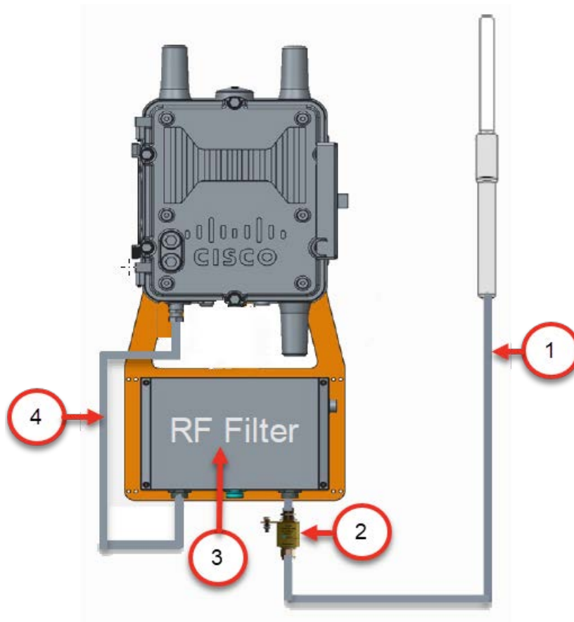
Figure 26 Remote Antenna, Lighting Arrestor Connections with a RF Filter
