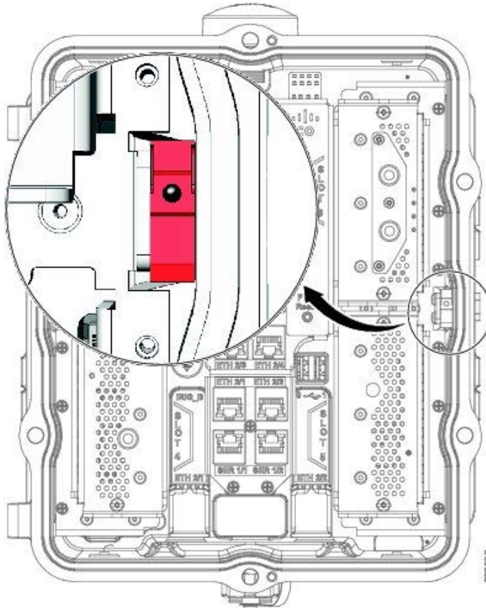
Figure 11 CGR's Door Sensor Location
