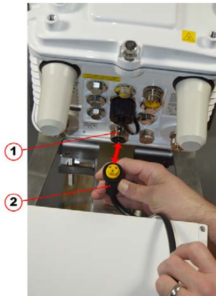
Figure 69 Power Input Connection on the CGR Location
