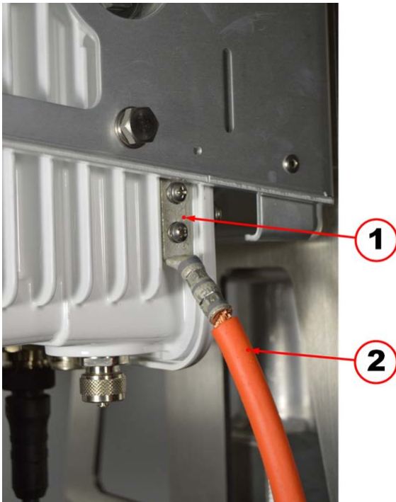
Figure 38 6AWG Ground Cable and Ground Lug Location
