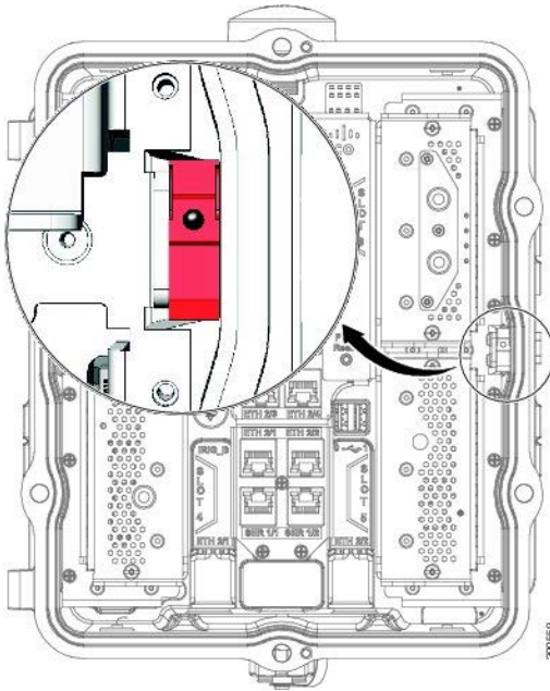
Figure 74 CGR's Door Sensor Location
