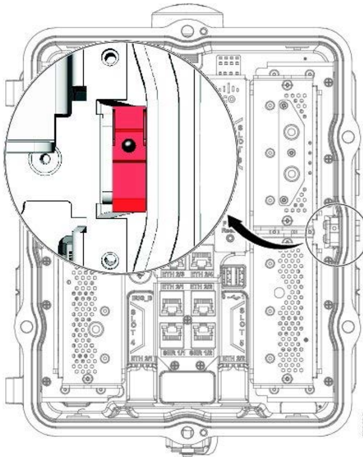
Figure 46 CGR's Door Sensor Location
