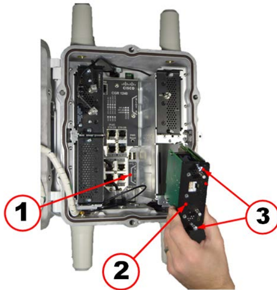
Figure 49 Slot 5 Label, CAMS3/CAM3M and Retaining Screws Location
