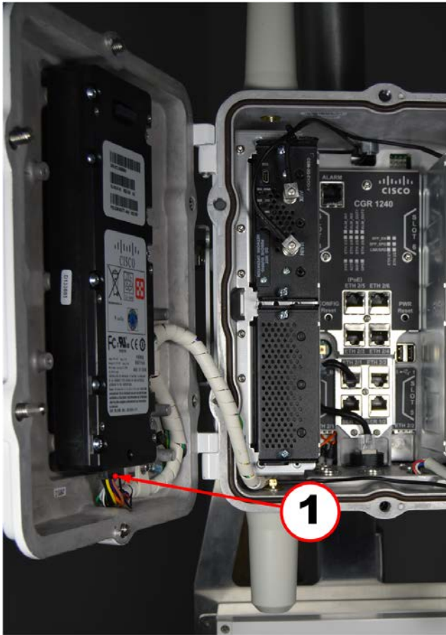
Figure 12 Battery Backup Unit (BBU) Harness Cable Connection Location
