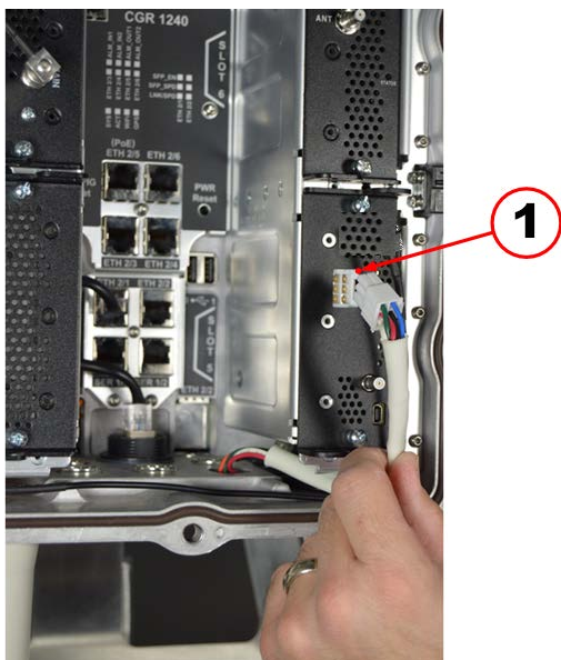
Figure 53 6-Pin Connector Location
