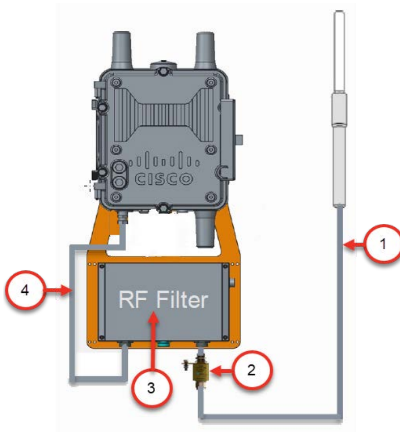
Figure 92 RF Filter Installation Configuration
