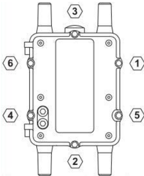
Figure 56 Six Bolt Sequence to Tighten the CGR's Door
