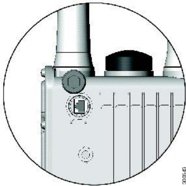
Figure 77 RJ45 Connector Location
