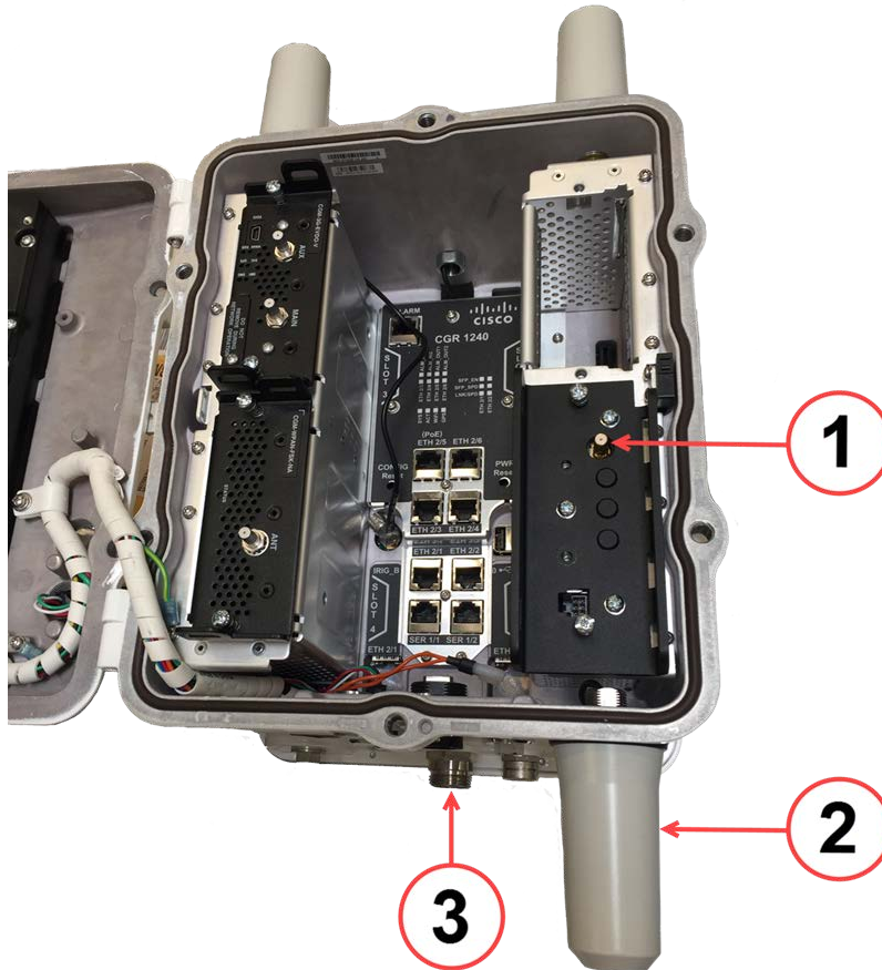
Figure 18 WPAN, Remote Antenna Connection and RF QMA Connector Location
