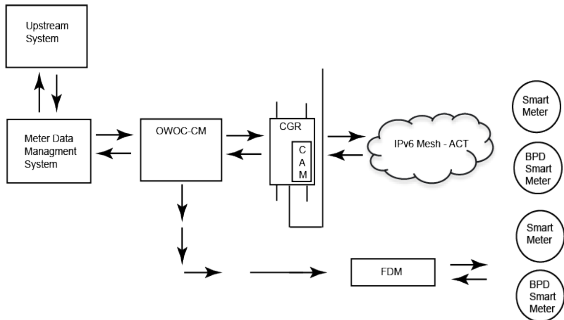
Figure 6 OpenWay Riva Communication Solution Network
