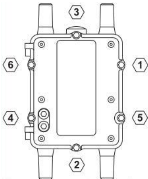
Figure 24 Six Captive Bolt Sequence to Tighten the CGR's Door
