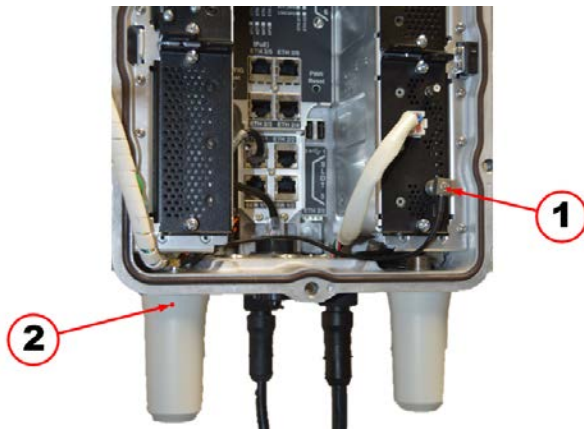
Figure 54 RF QMA Connector and WPAN Antenna Connection Location
