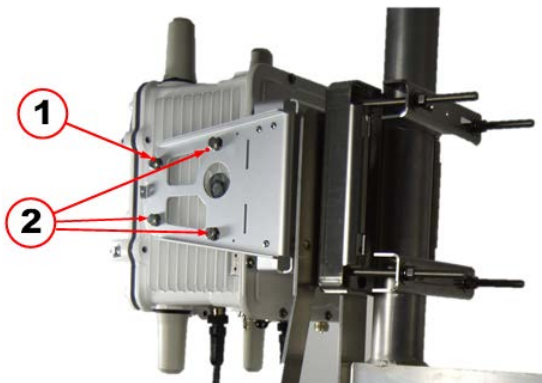
Figure 23 Hex Bolts Location on Side of CGR
