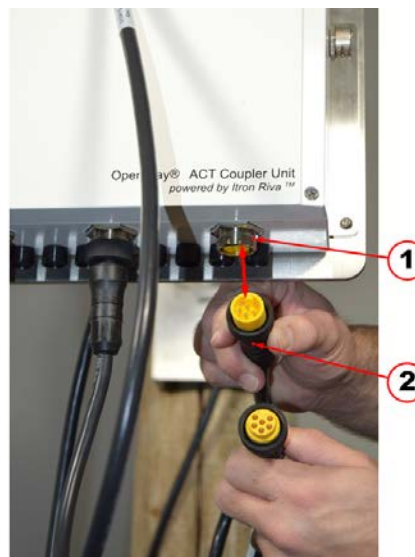
Figure 70 PLC Signal Cable Connection on the ACT Coupler Unit Location
