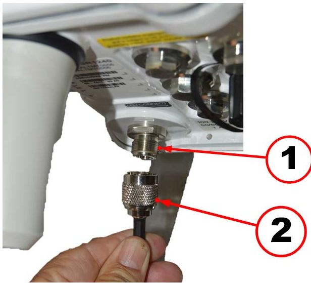
Figure 93 RF Filer to CGR Connection
