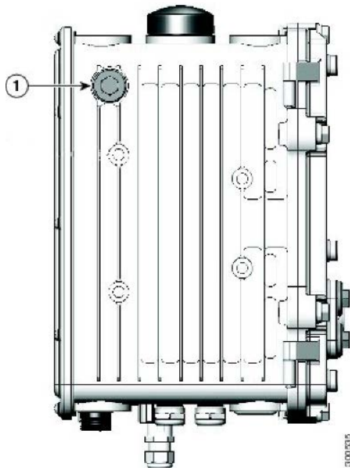
Figure 75 Hex Bolt Plug - RJ45 Connector Location
