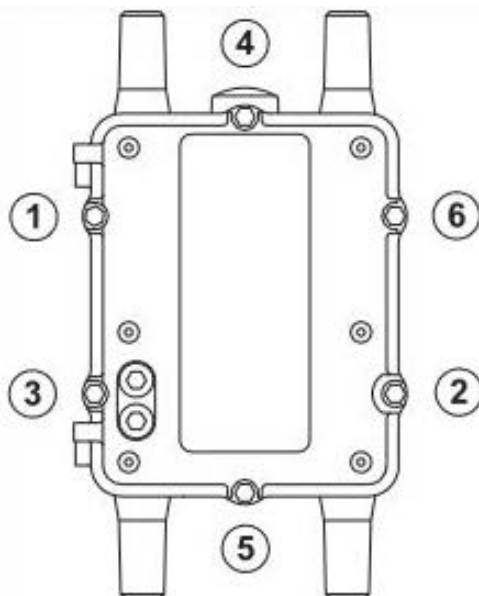
Figure 10 Six Captive Bolt Sequence to Loosen the CGR's Door
