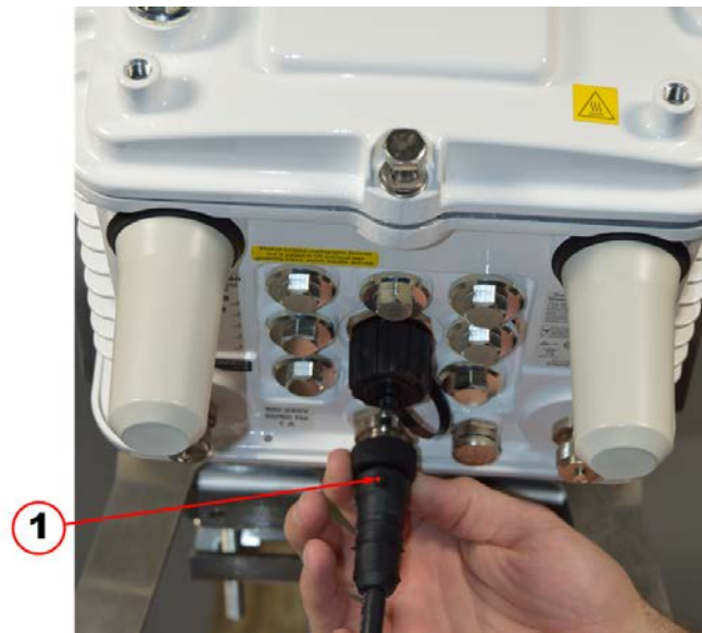
Figure 39 AC Power Cable Connection Location
