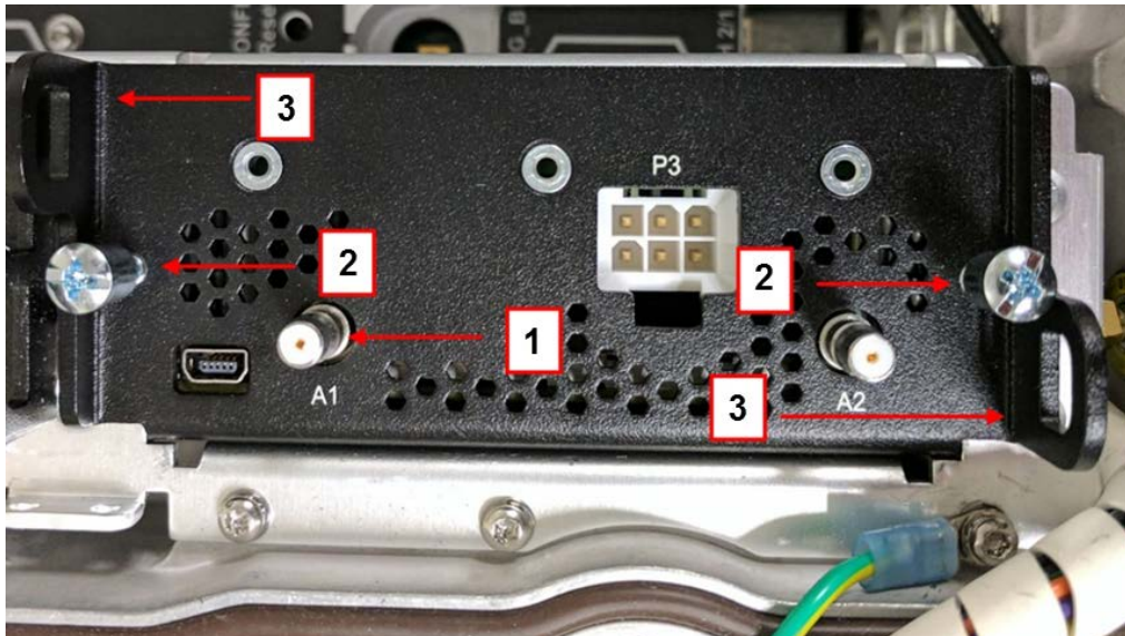
Figure 83 CAM Handles, Phillips Screws and RF QMA Connector Location
