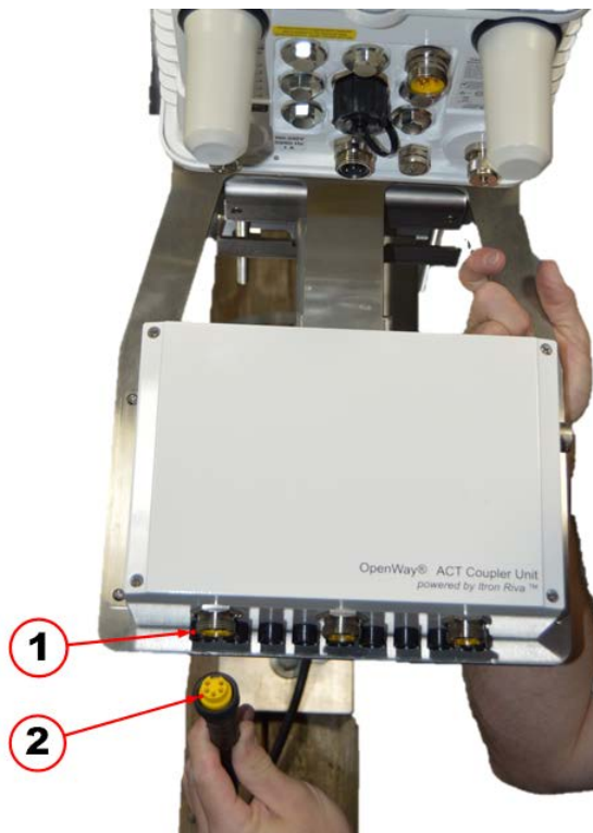
Figure 65 AC Power Connection Location
