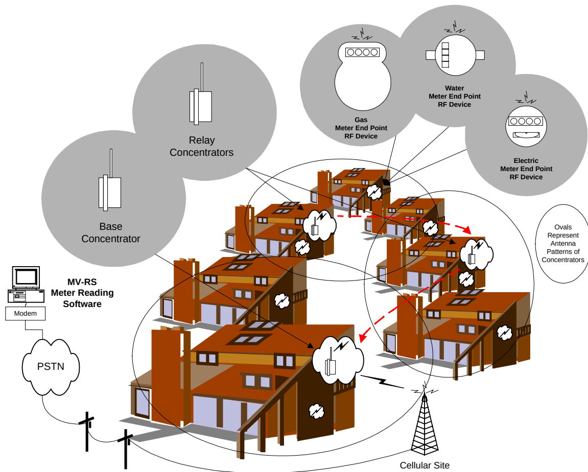
Figure 1 - Basic Components of Itron's Submetering Network
