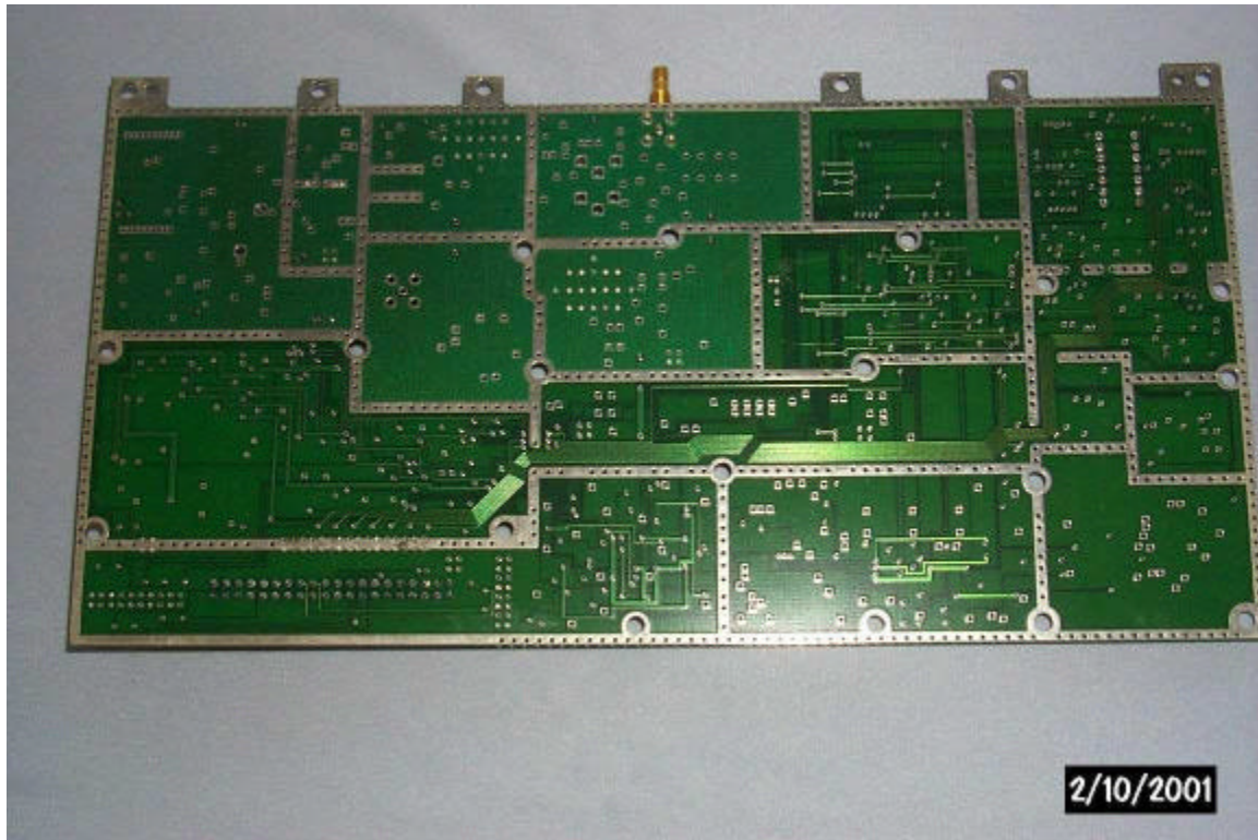
RF PCB REAR
