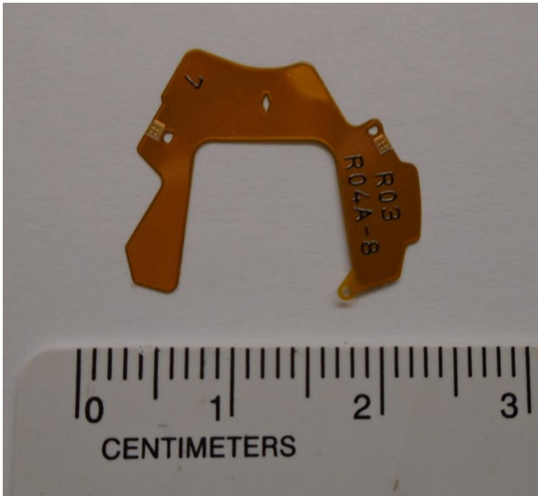
unfolded 2.4 GHz antenna
