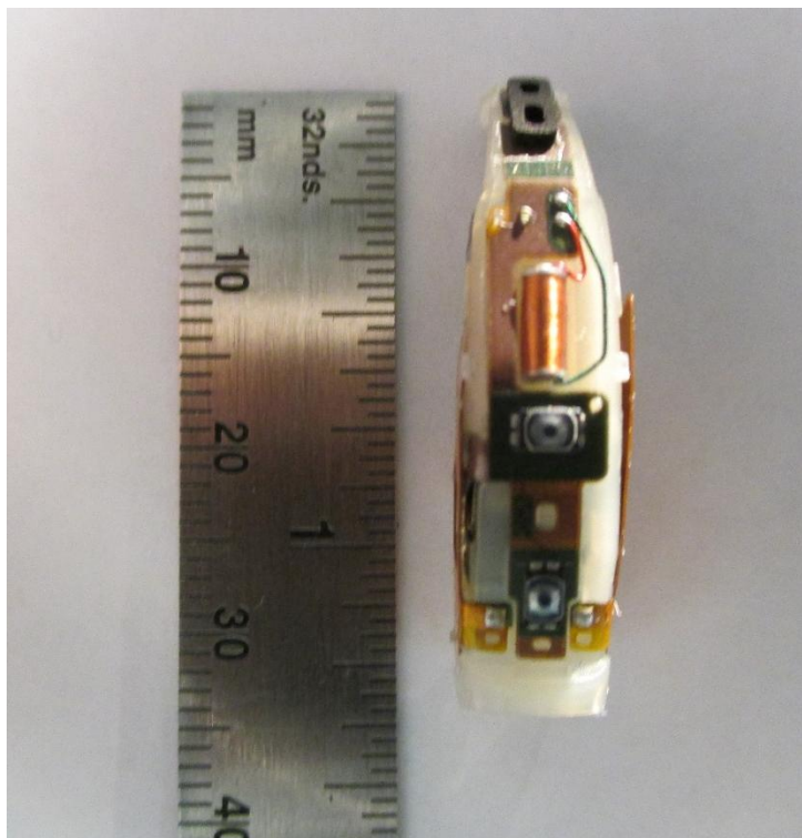
top and receiver end without ear tube
