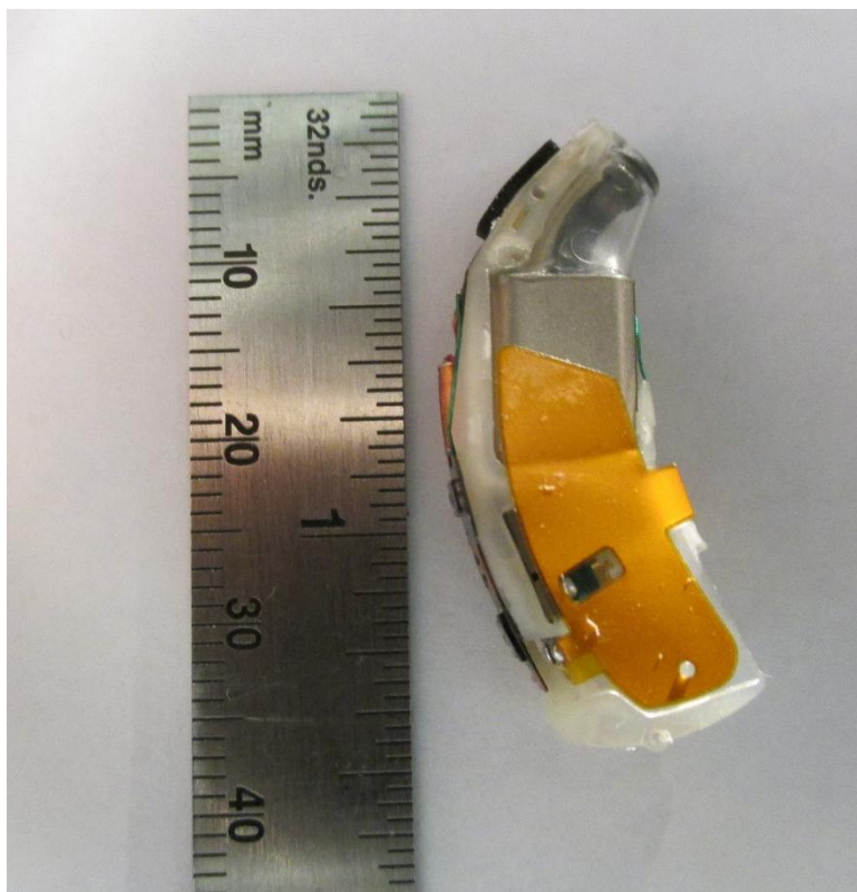
Right side with antenna
