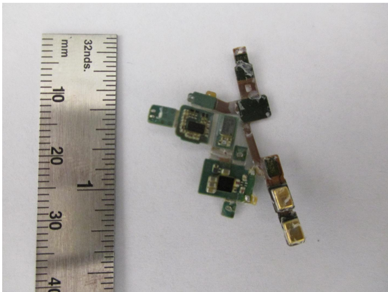
Unfolded flex circuit top view
