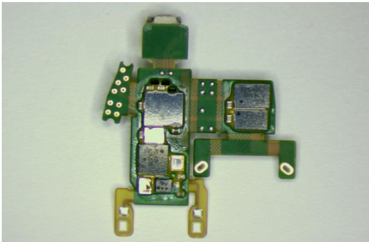
Bottom view of flex circuit
