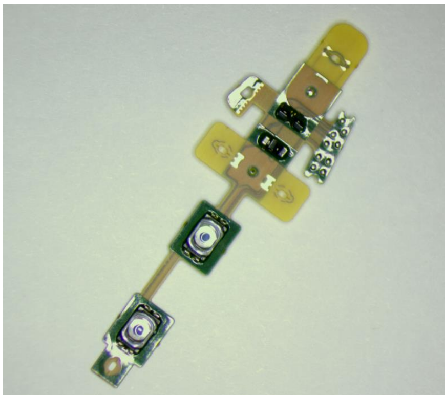
bottom view of mic flex
