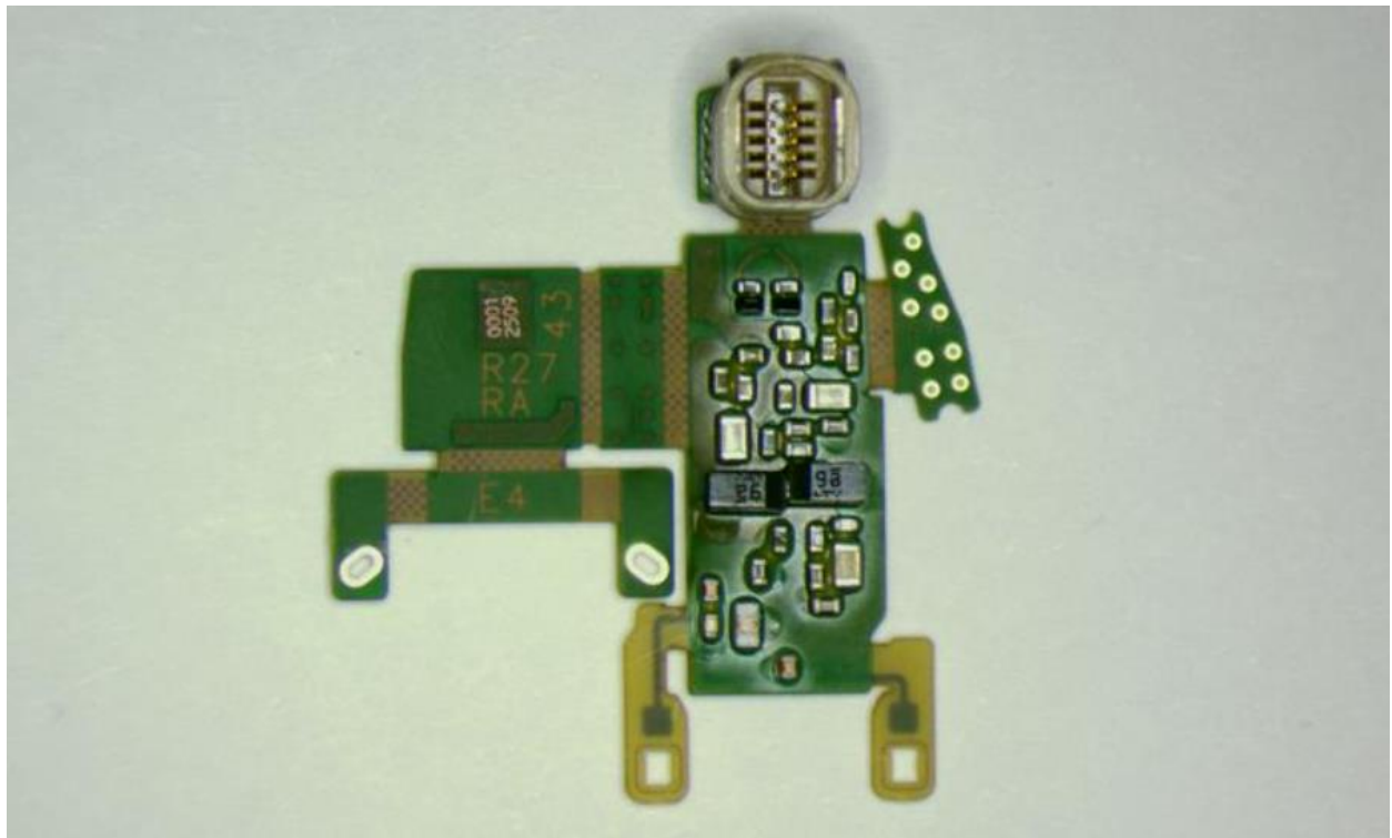
Unfolded flex circuit top view
