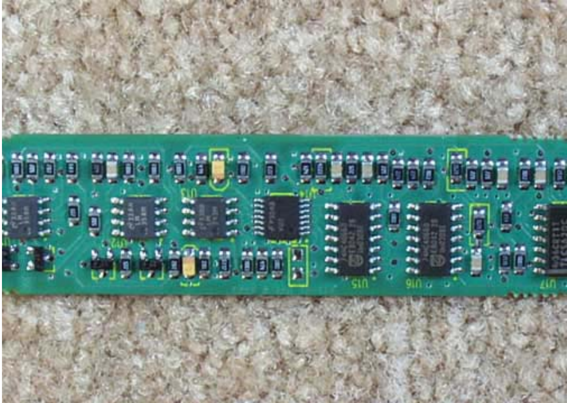
Audio PCB Front Closeup 2
