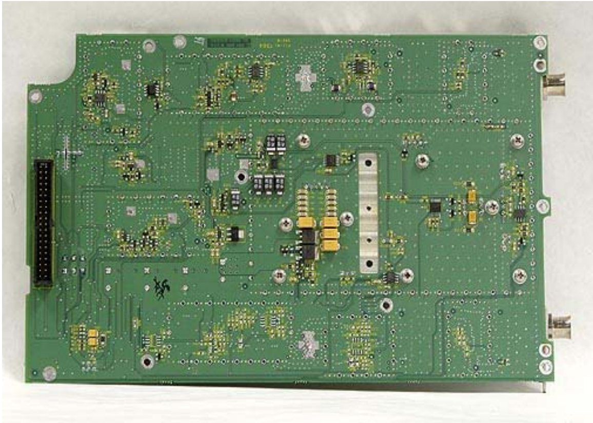
RF Board 2
