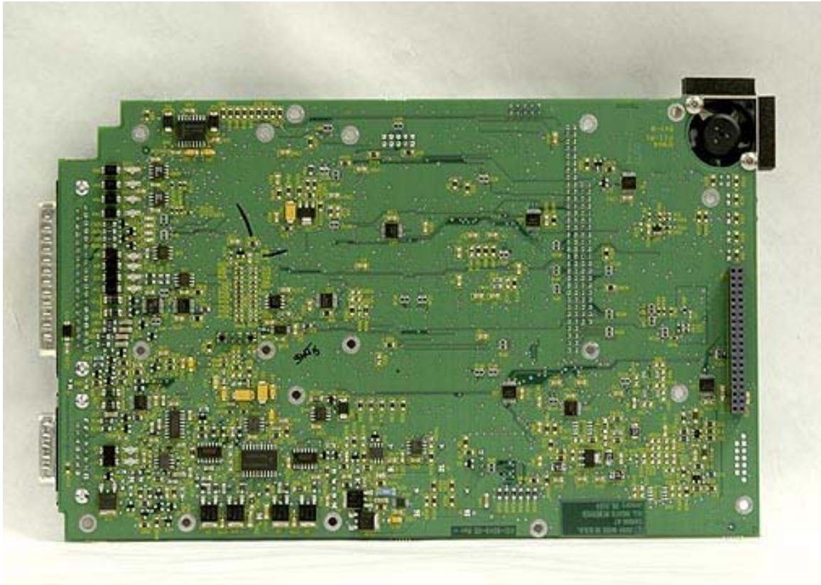
Main Logic Board 2
