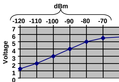
Figure 18 - T855 and T885, Typical RSSI Curve: volt to dBm
