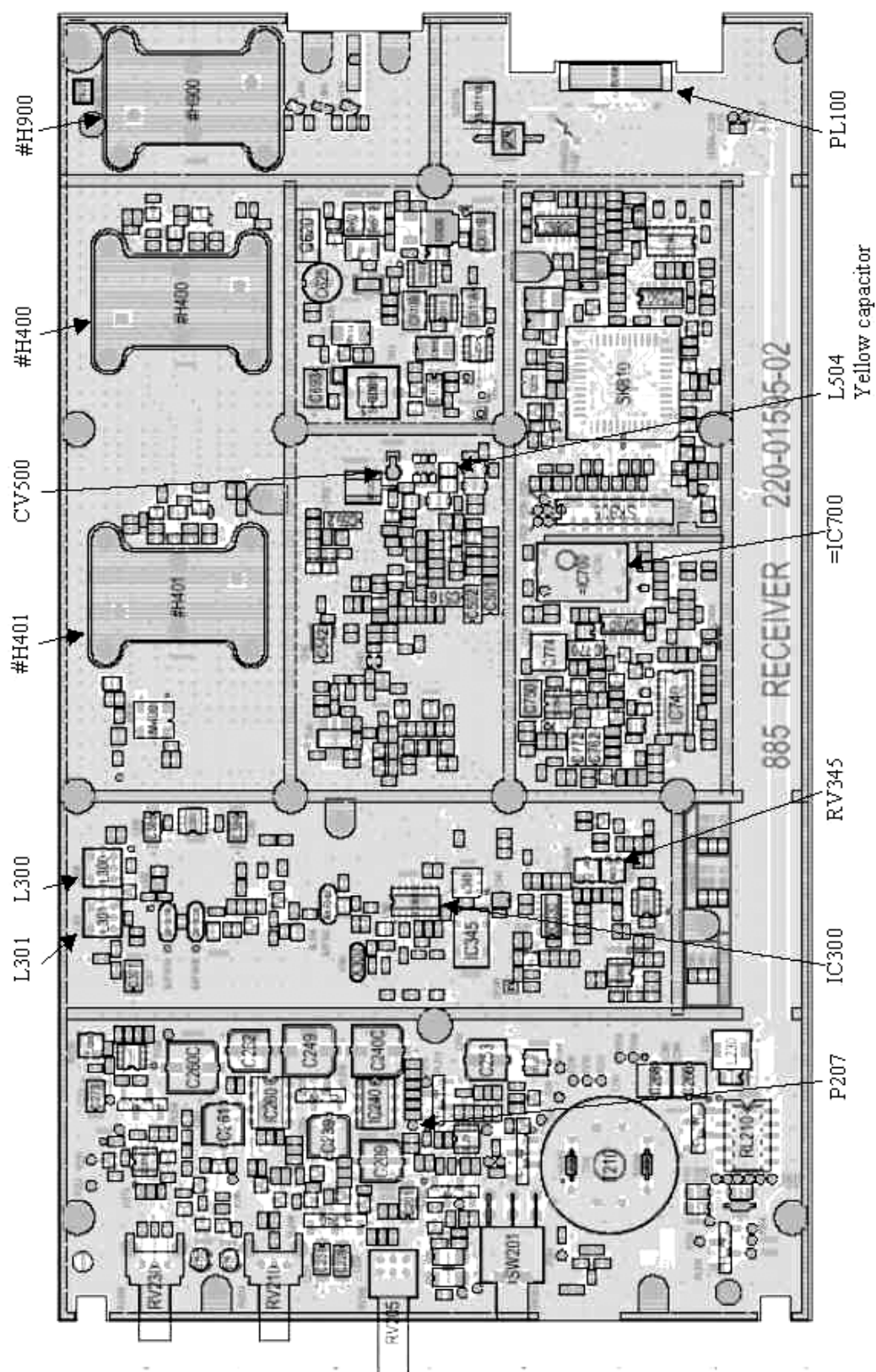
Figure 20 - T885-0200 Receiver Tuning Controls location
