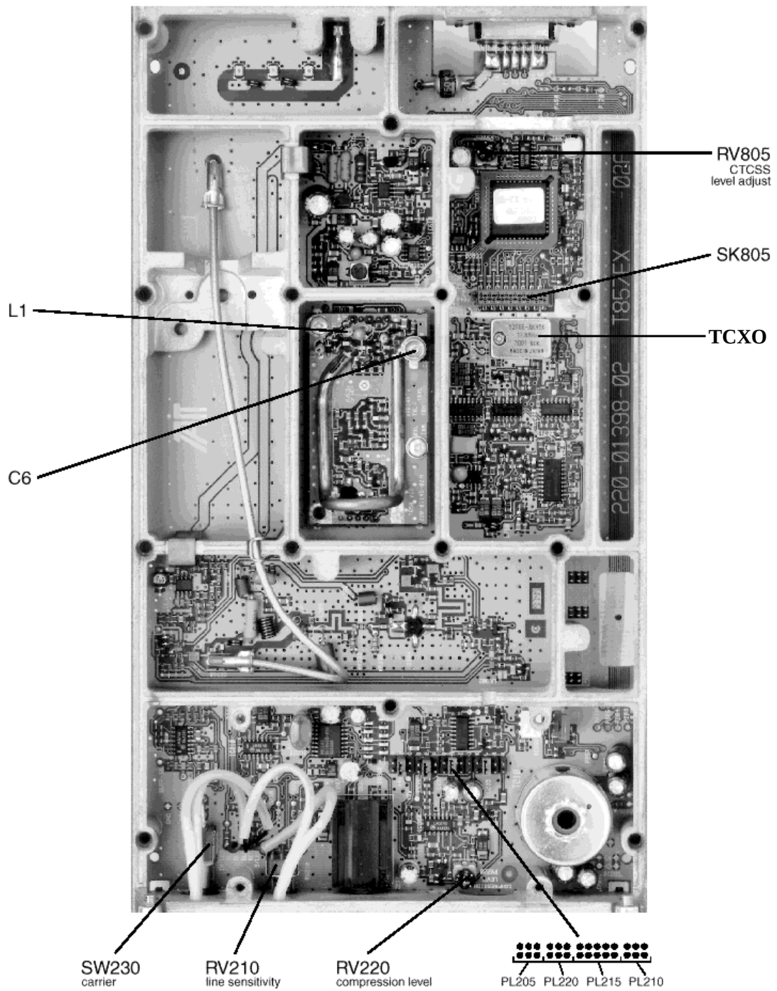
Figure 30 - T857 Exciter Tuning Controls Locations
