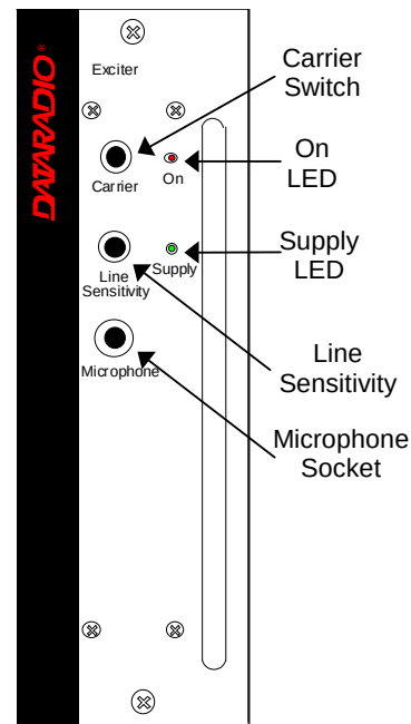
Figure 7 - Exciter module, front panel
