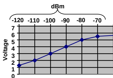
Figure 22 - T855 and T885, Typical RSSI Curve: volt to dBm
