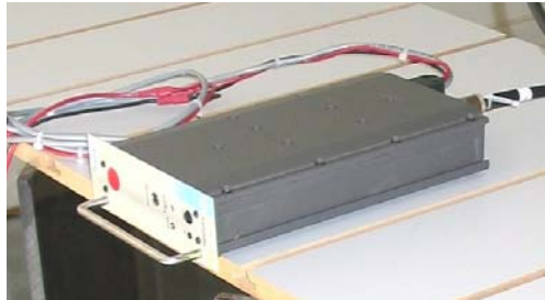
DataRadio T881-10 700 MHz band base station tested for radiated spurious emissions
