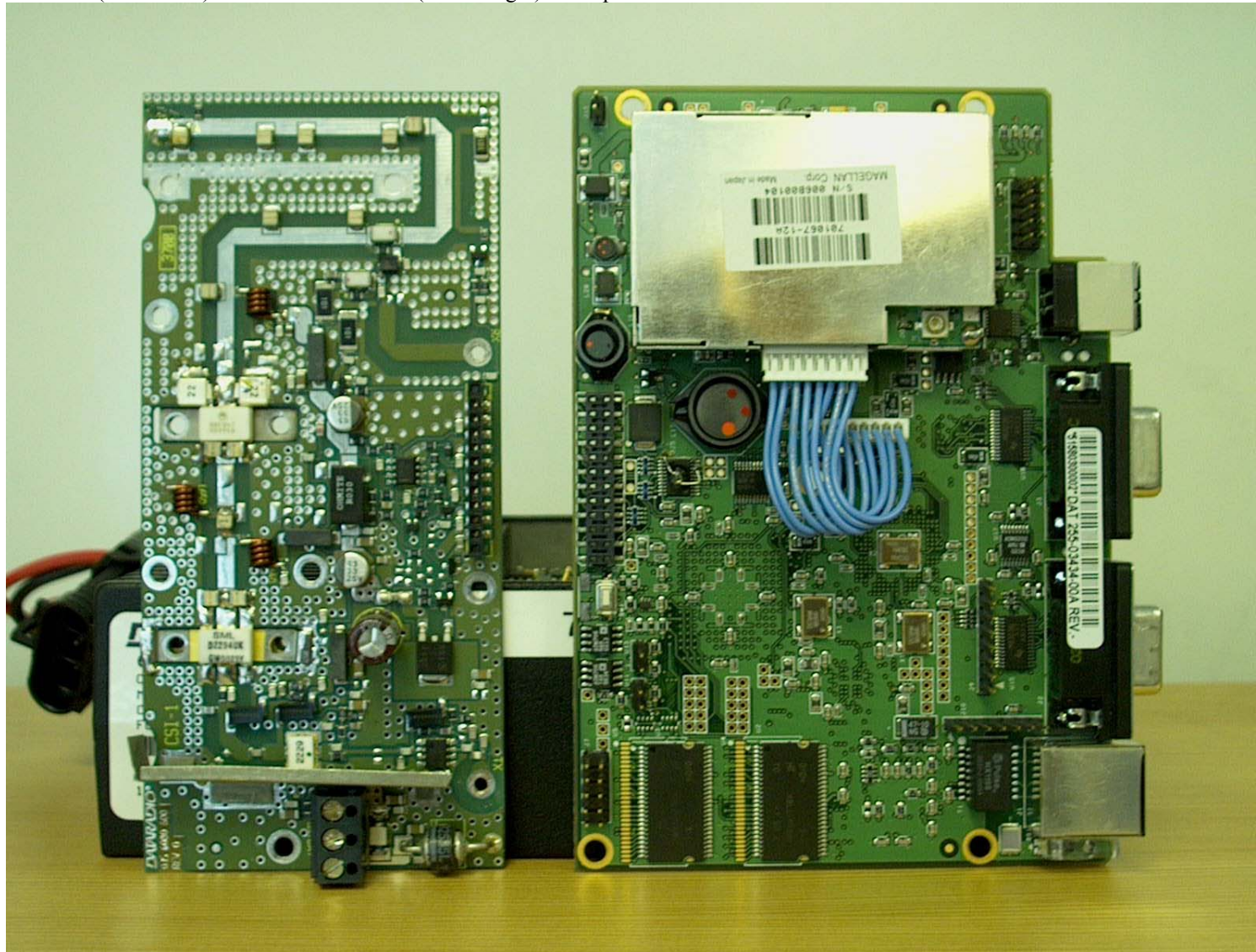
PA board (toward left) and G3 modem board (toward right) – component side
