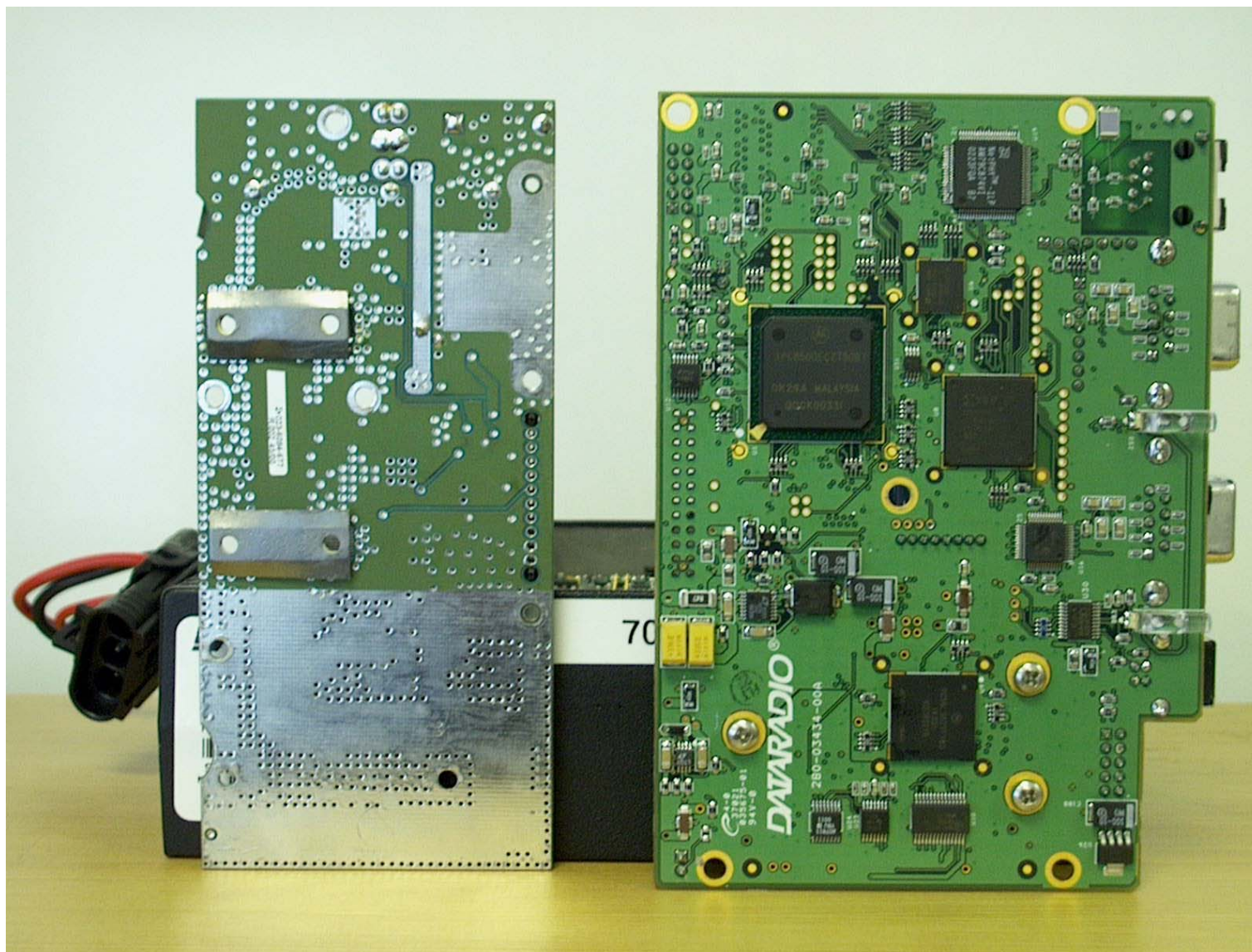
PA board (toward left) and G3 modem board (toward right) – soldering side
