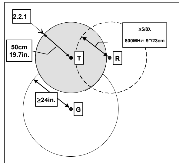
Figure 4 - Antenna spacing
