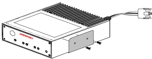
Figure 2 - Bracket installation
