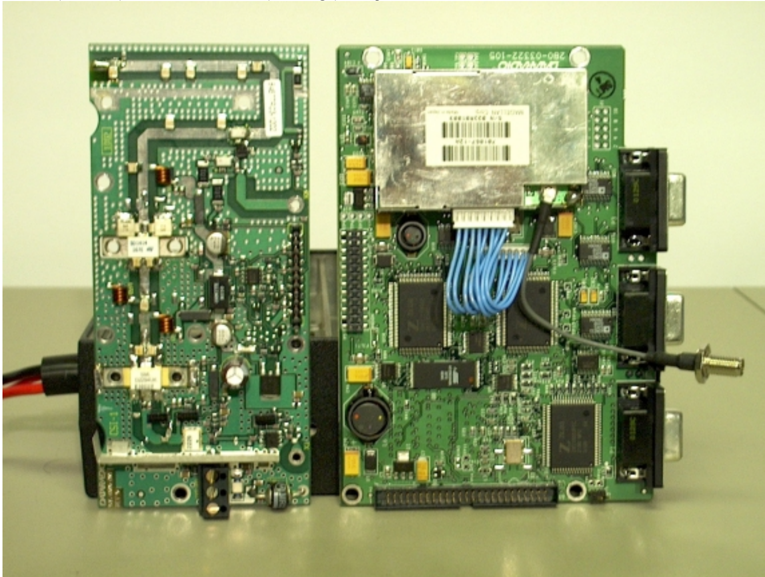
PA board (toward left) and GCU2 modem board (toward right) – component side
