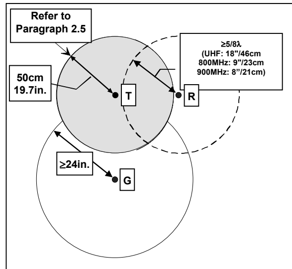
Figure 4 - Antenna spacing
