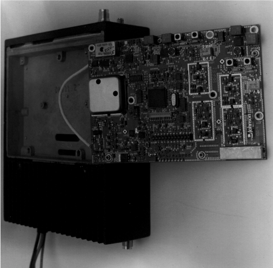
Figure 6 Internal bottom view, service position
