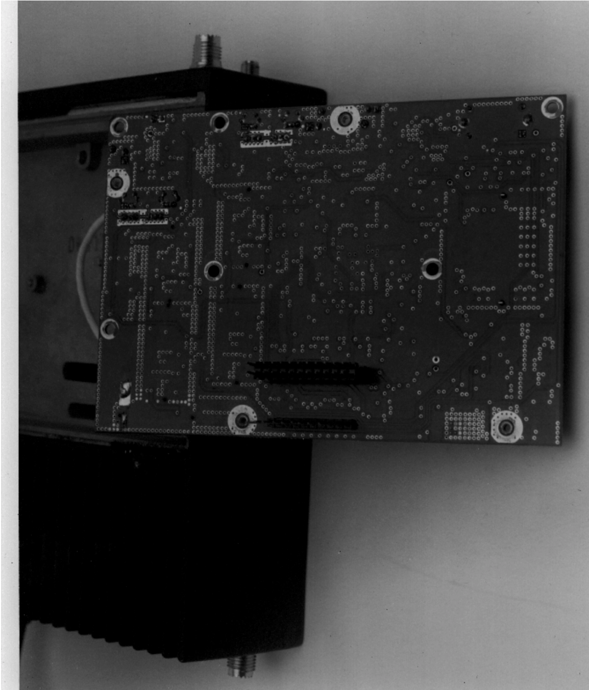
Figure 5 Internal, bottom view, hidden side
