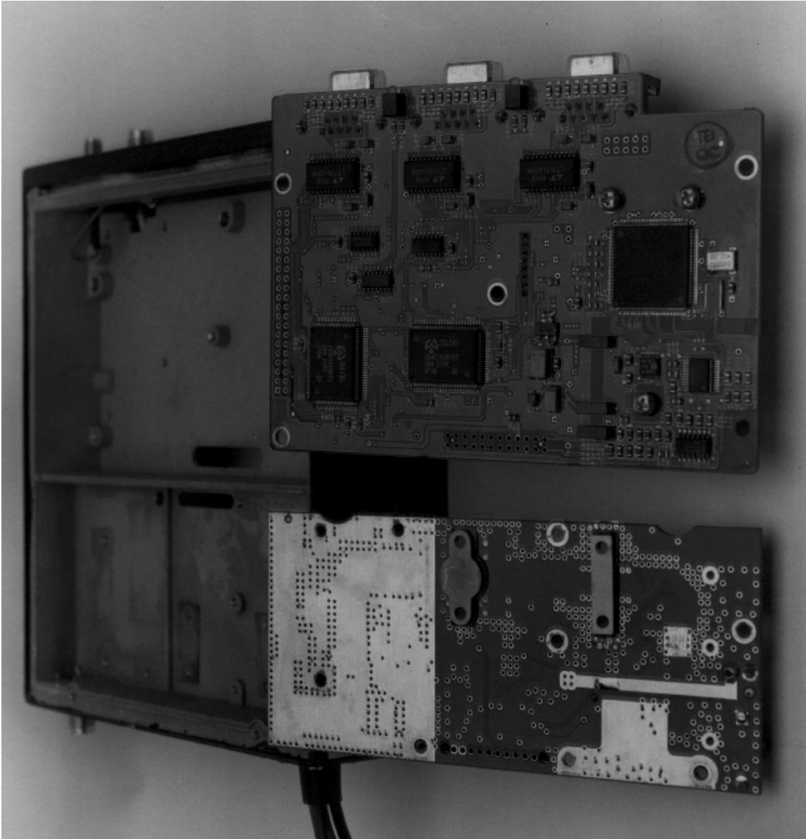
Figure 4 Internal top view, hidden side
