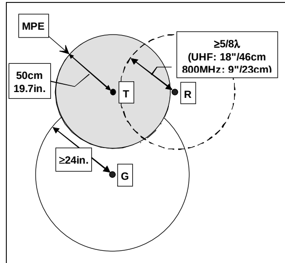
Figure 4 - Antenna spacing
