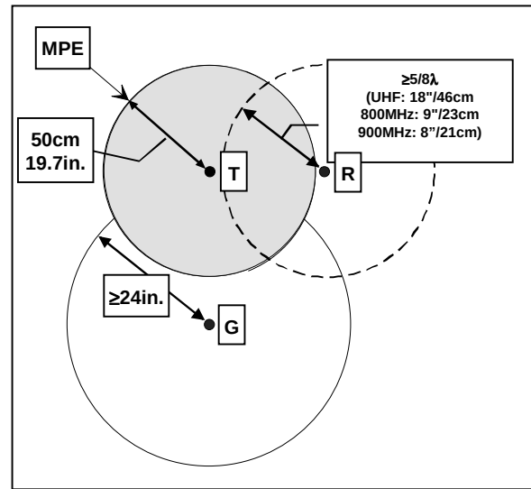
Figure 4 - Antenna spacing
