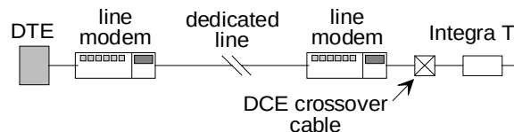
Figure 4 - Tail Circuit
