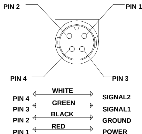
Figure 11- Power / Analog cable
