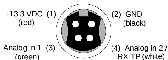
Figure 10 - Power / Analog Connector
