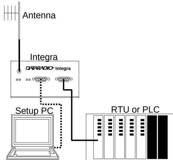
Figure 1 - Basic connections required
