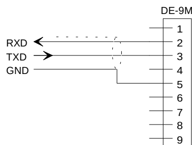
Figure 8 – 3-wire interface
