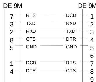
Figure 5 - DCE Crossover Cable for RTS-CTS mode
