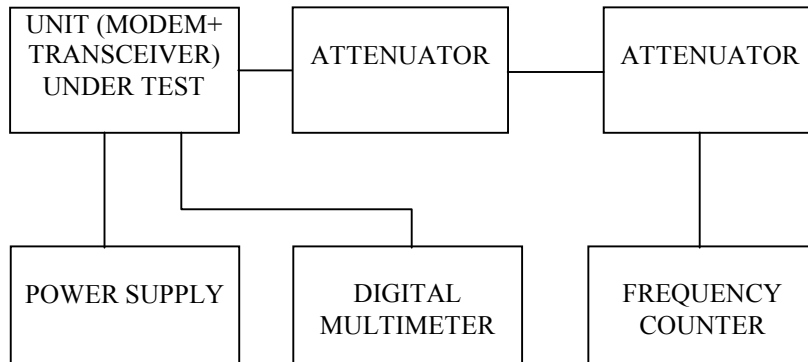
TEST SET-UP
