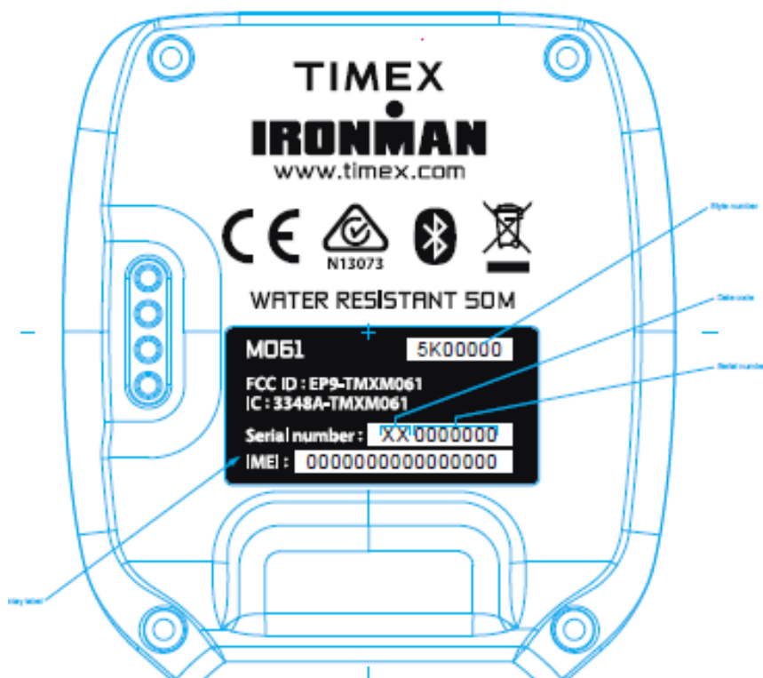
Figure 1-1 Label information
