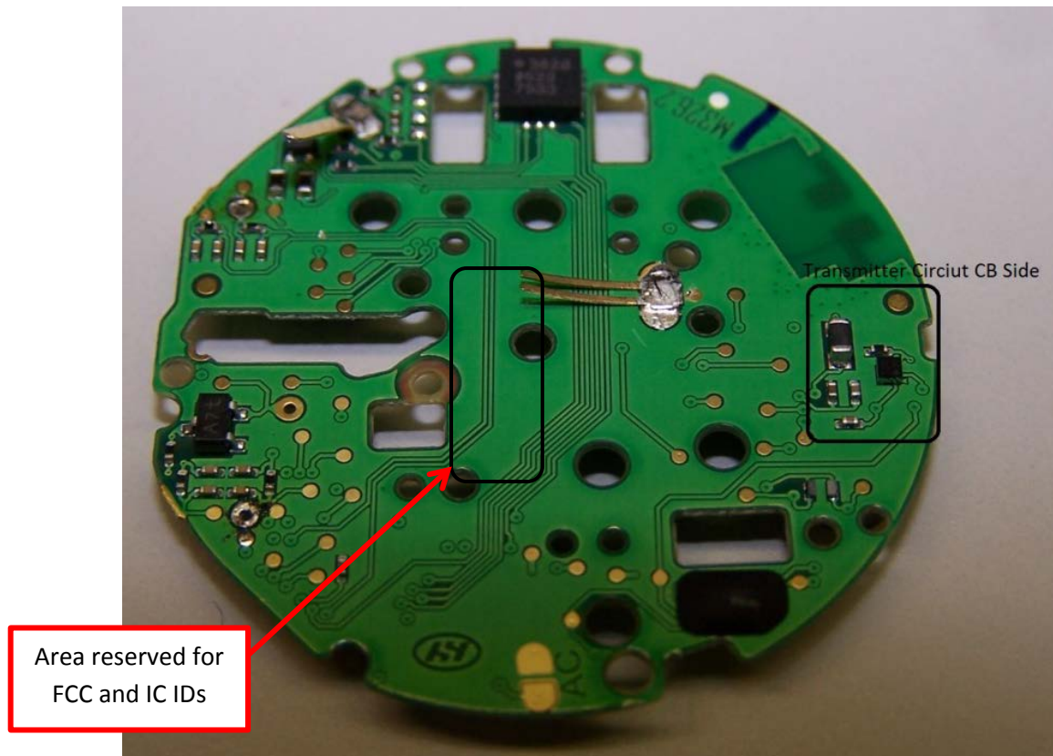
Figure 2: Location of ID label
