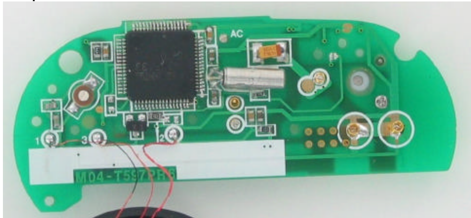
PCB opposite side
