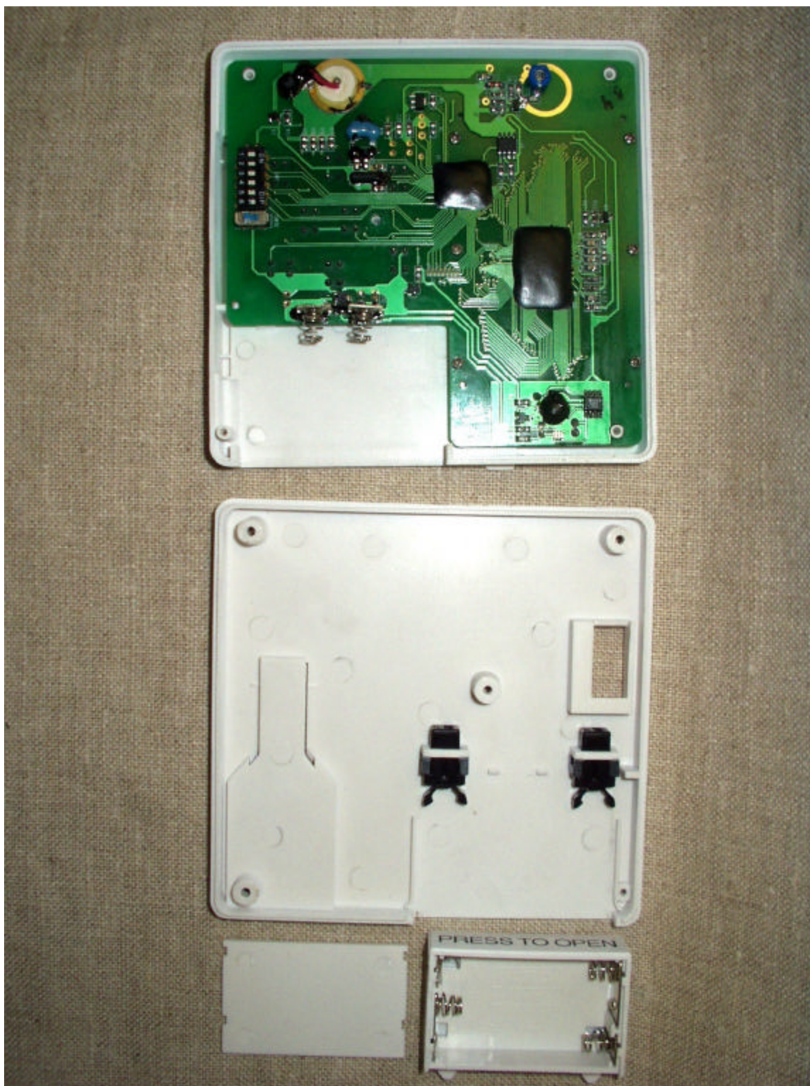
Photograph: 1 Overview – Inside Chassis WMT
