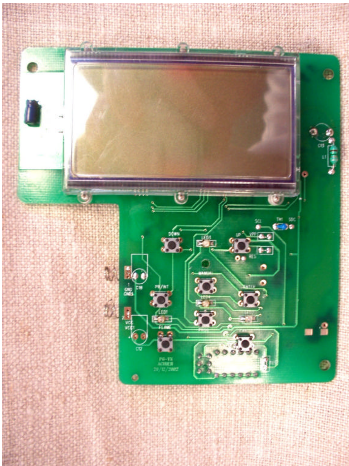
Photograph: 4 PCB – Display Side WMT
