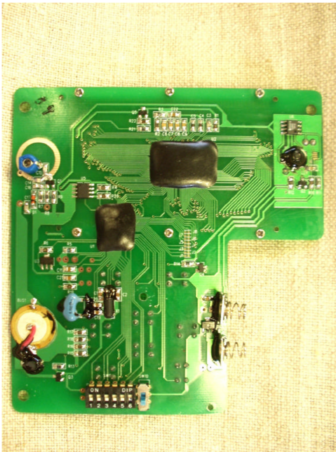
Photograph: 3 PCB – Component Side WMT
