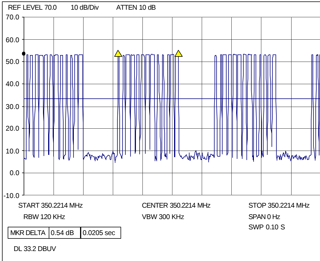
Figure 4-3: Output – 100 milliseconds
