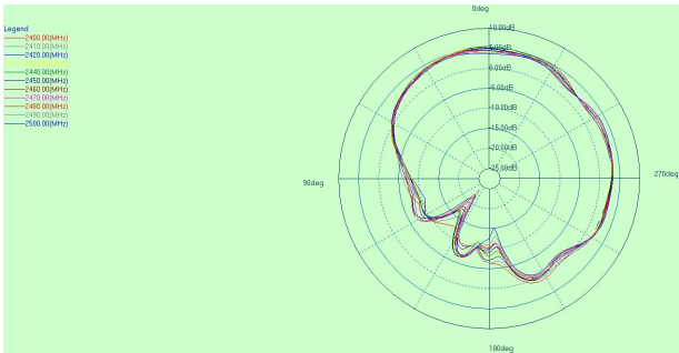
2.4G phi=90deg
