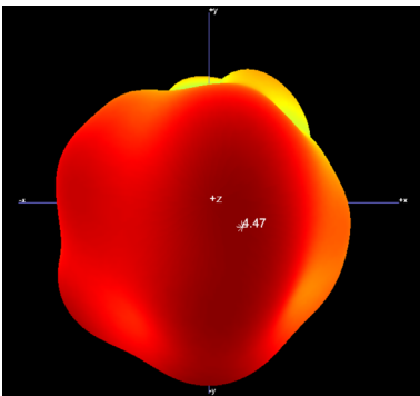
2.4G 3D
