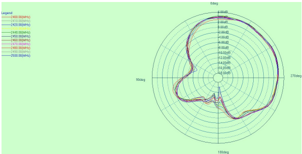
2.4G phi=90deg
