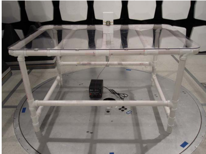
Worst-case radiated emission, front view
